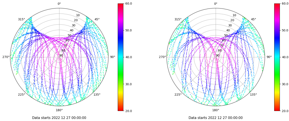
Skyplot for station IZAN. Signal to Noise S1C Data file IZAN00ESP_R_2022361.xtr Skyplot for station IZAN. Signal to Noise S2S Data file IZAN00ESP_R_2022361.xtr
