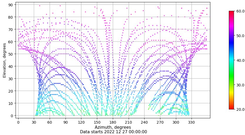
Azimuth-elevation plot for station IZAN. Signal to Noise S1C Data file IZAN00ESP_R_2022361.xtr
