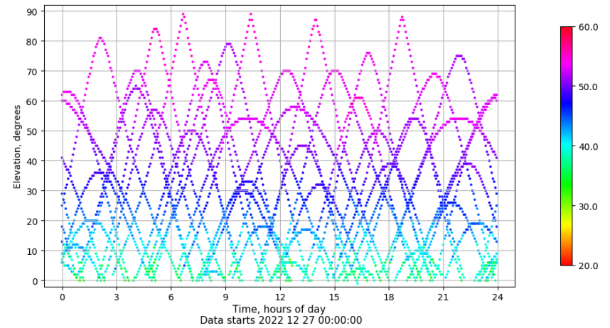
Time-elevation plot for station IZAN. Signal to Noise S1C Data file IZAN00ESP_R_2022361.xtr
