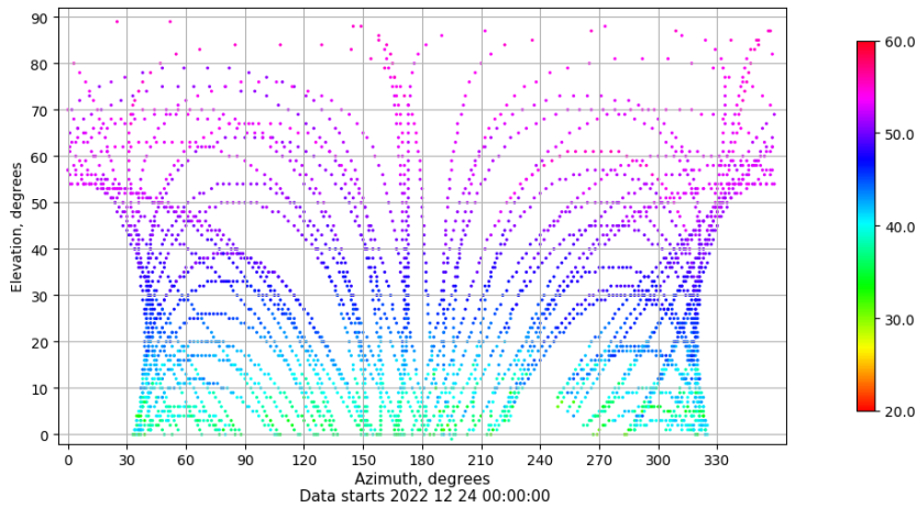
Azimuth-elevation plot for station IZAN. Signal to Noise S1C Data file IZAN00ESP_R_2022358.xtr
