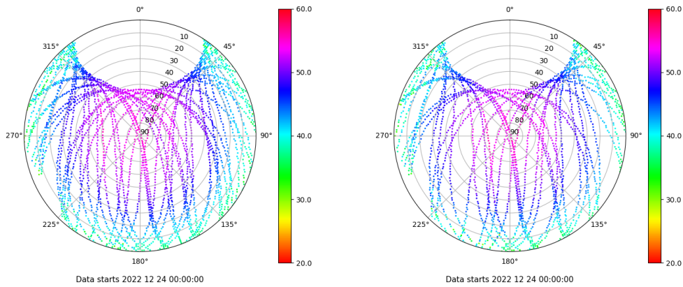
Skyplot for station IZAN. Signal to Noise S1C Data file IZAN00ESP_R_2022358.xtr Skyplot for station IZAN. Signal to Noise S2S Data file IZAN00ESP_R_2022358.xtr
