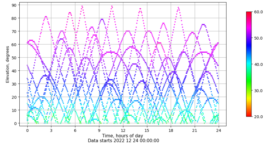
Time-elevation plot for station IZAN. Signal to Noise S1C Data file IZAN00ESP_R_2022358.xtr
