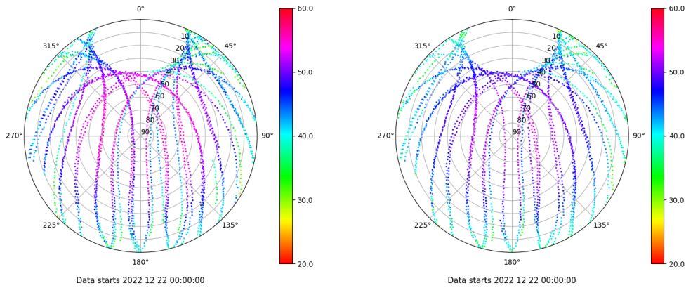
Skyplot for station IZAN. Signal to Noise S1C Data file IZAN00ESP_R_2022356.xtr Skyplot for station IZAN. Signal to Noise S2C Data file IZAN00ESP_R_2022356.xtr
