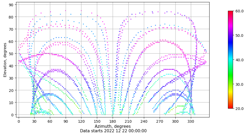
Azimuth-elevation plot for station IZAN. Signal to Noise S1C Data file IZAN00ESP_R_2022356.xtr
