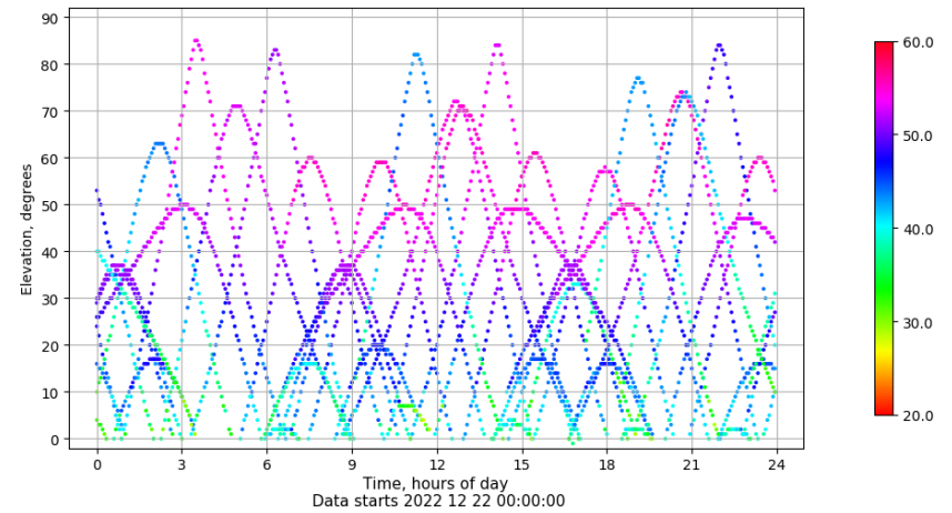
Time-elevation plot for station IZAN. Signal to Noise S1C Data file IZAN00ESP_R_2022356.xtr
