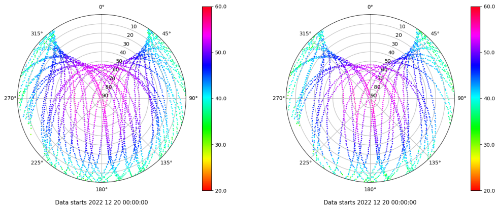
Skyplot for station IZAN. Signal to Noise S1C Data file IZAN00ESP_R_2022354.xtr Skyplot for station IZAN. Signal to Noise S2S Data file IZAN00ESP_R_2022354.xtr
