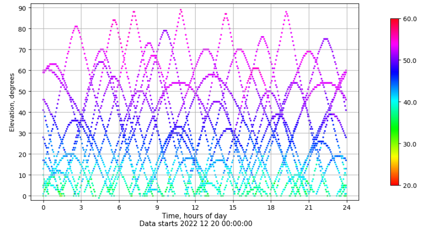
Time-elevation plot for station IZAN. Signal to Noise S1C Data file IZAN00ESP_R_2022354.xtr
