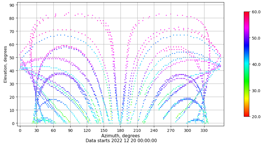
Azimuth-elevation plot for station IZAN. Signal to Noise S1C Data file IZAN00ESP_R_2022354.xtr
