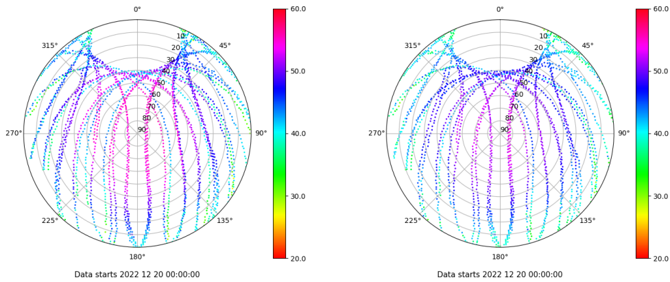
Skyplot for station IZAN. Signal to Noise S1C Data file IZAN00ESP_R_2022354.xtr Skyplot for station IZAN. Signal to Noise S2C Data file IZAN00ESP_R_2022354.xtr
