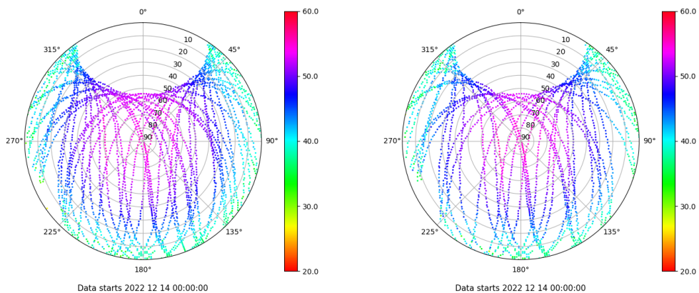
Skyplot for station IZAN. Signal to Noise S1C Data file IZAN00ESP_R_2022348.xtr Skyplot for station IZAN. Signal to Noise S2S Data file IZAN00ESP_R_2022348.xtr
