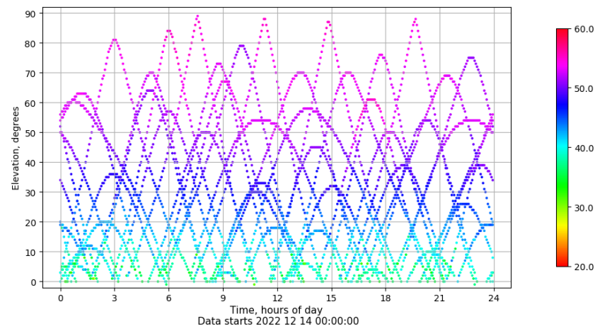
Time-elevation plot for station IZAN. Signal to Noise S1C Data file IZAN00ESP_R_2022348.xtr
