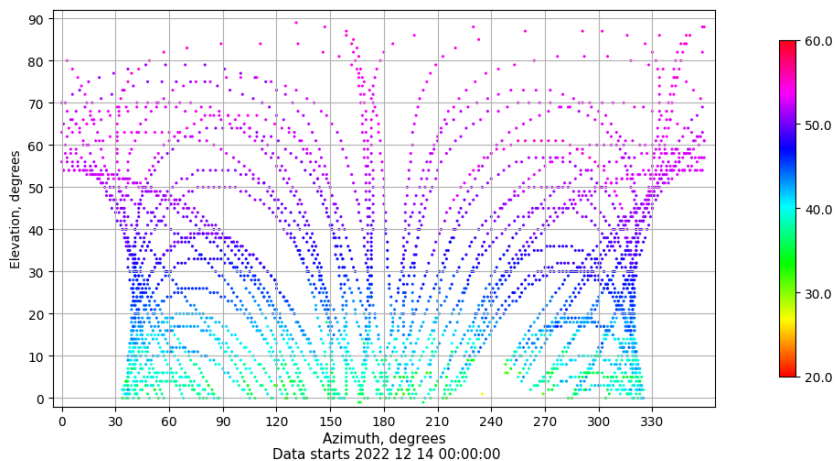
Azimuth-elevation plot for station IZAN. Signal to Noise S1C Data file IZAN00ESP_R_2022348.xtr
