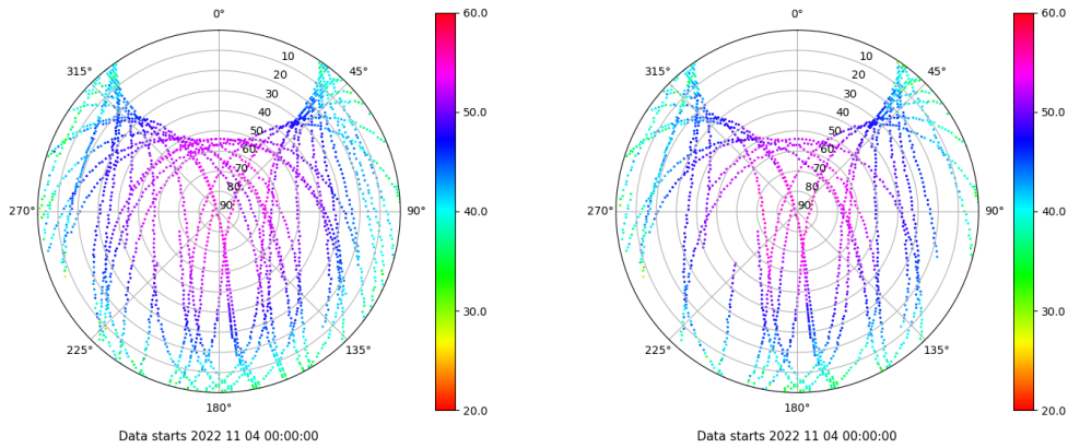
Skyplot for station IZAN. Signal to Noise S1C Data file IZAN00ESP_R_2022308.xtr Skyplot for station IZAN. Signal to Noise S2S Data file IZAN00ESP_R_2022308.xtr
