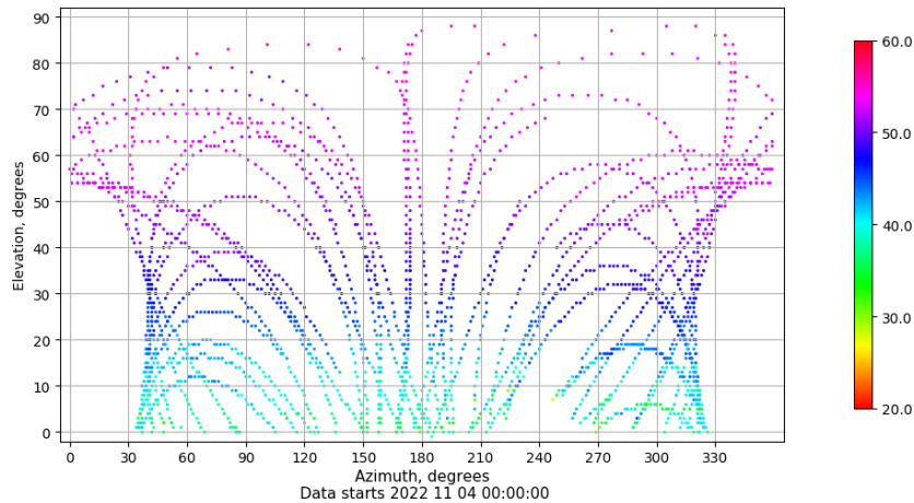
Azimuth-elevation plot for station IZAN. Signal to Noise S1C Data file IZAN00ESP_R_2022308.xtr
