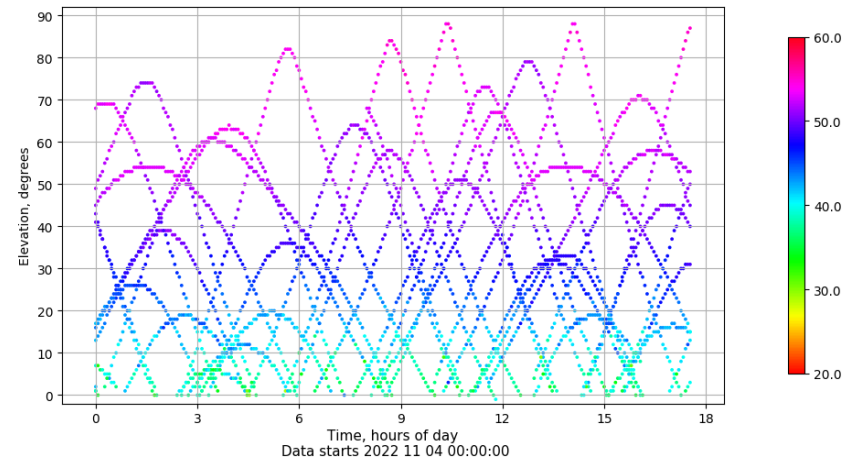
Time-elevation plot for station IZAN. Signal to Noise S1C Data file IZAN00ESP_R_2022308.xtr
