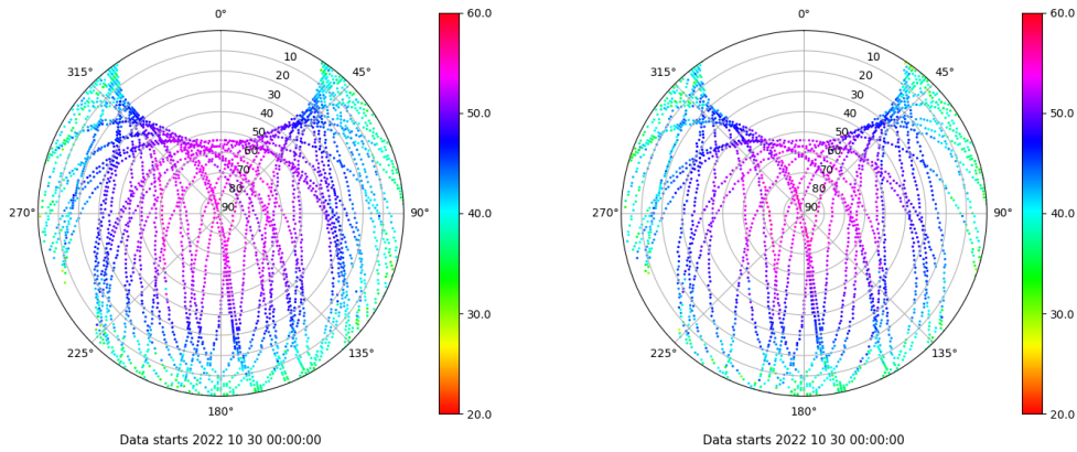
Skyplot for station IZAN. Signal to Noise S1C Data file IZAN00ESP_R_2022303.xtr Skyplot for station IZAN. Signal to Noise S2S Data file IZAN00ESP_R_2022303.xtr
