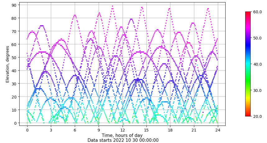
Time-elevation plot for station IZAN. Signal to Noise S1C Data file IZAN00ESP_R_2022303.xtr
