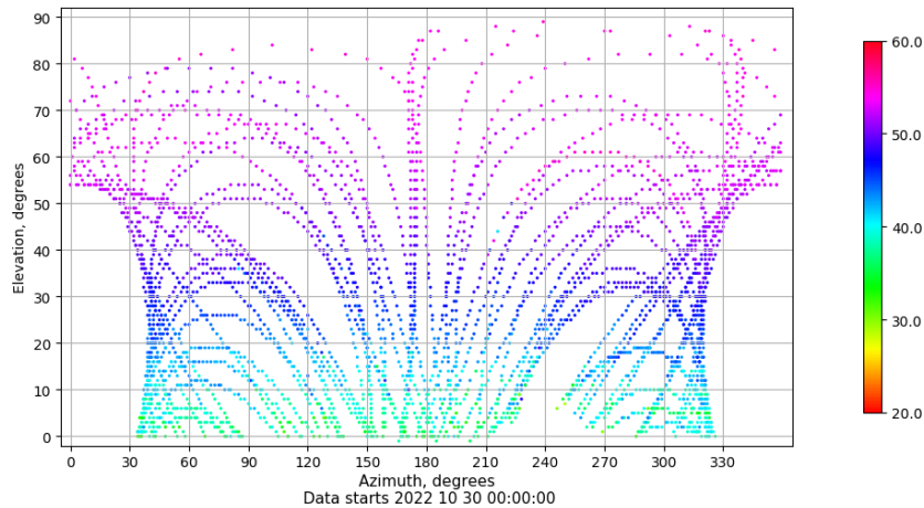
Azimuth-elevation plot for station IZAN. Signal to Noise S1C Data file IZAN00ESP_R_2022303.xtr
