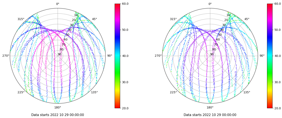
Skyplot for station IZAN. Signal to Noise S1C Data file IZAN00ESP_R_2022302.xtr Skyplot for station IZAN. Signal to Noise S2C Data file IZAN00ESP_R_2022302.xtr
