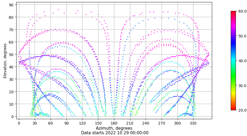
Azimuth-elevation plot for station IZAN. Signal to Noise S1C Data file IZAN00ESP_R_2022302.xtr
