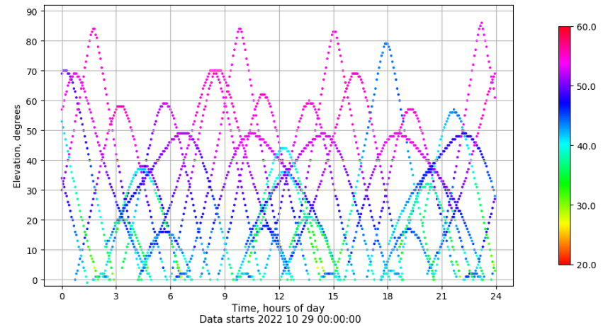
Time-elevation plot for station IZAN. Signal to Noise S1C Data file IZAN00ESP_R_2022302.xtr
