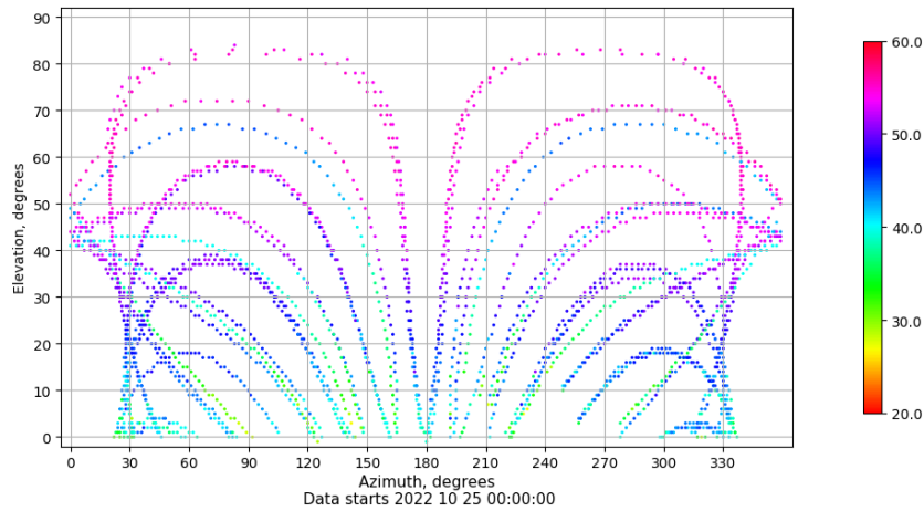
Azimuth-elevation plot for station IZAN. Signal to Noise S1C Data file IZAN00ESP_R_2022298.xtr
