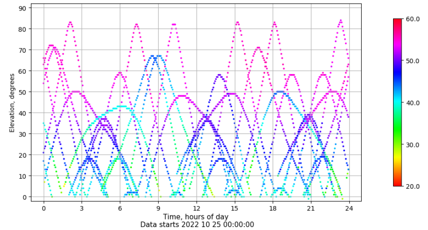
Time-elevation plot for station IZAN. Signal to Noise S1C Data file IZAN00ESP_R_2022298.xtr
