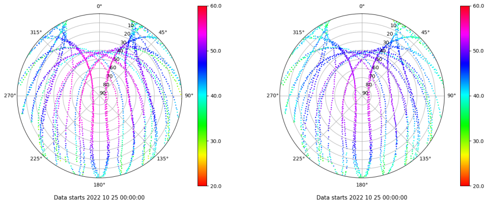
Skyplot for station IZAN. Signal to Noise S1C Data file IZAN00ESP_R_2022298.xtr Skyplot for station IZAN. Signal to Noise S2C Data file IZAN00ESP_R_2022298.xtr
