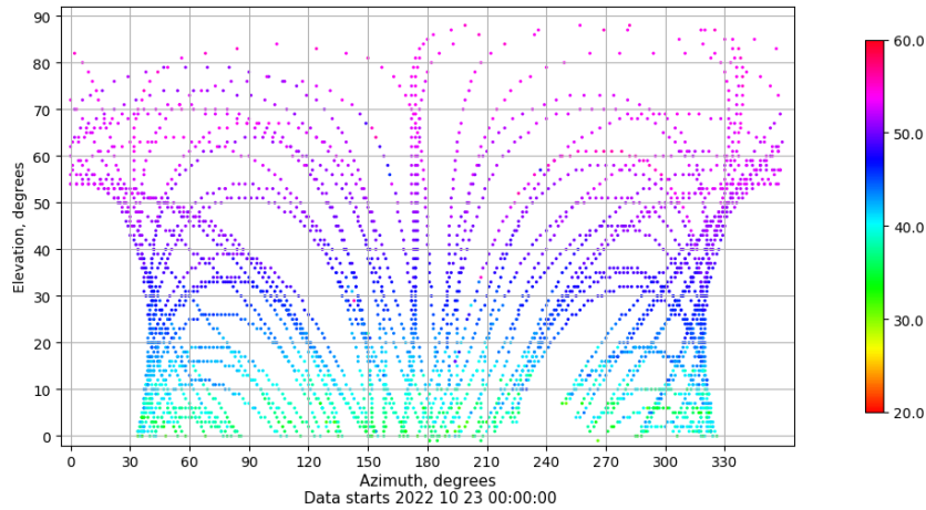
Azimuth-elevation plot for station IZAN. Signal to Noise S1C Data file IZAN00ESP_R_2022296.xtr
