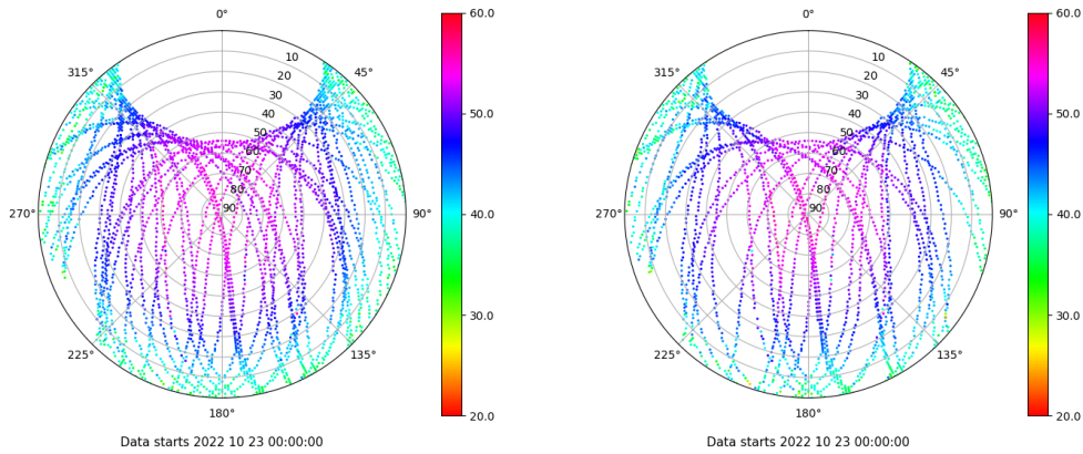
Skyplot for station IZAN. Signal to Noise S1C Data file IZAN00ESP_R_2022296.xtr Skyplot for station IZAN. Signal to Noise S2S Data file IZAN00ESP_R_2022296.xtr
