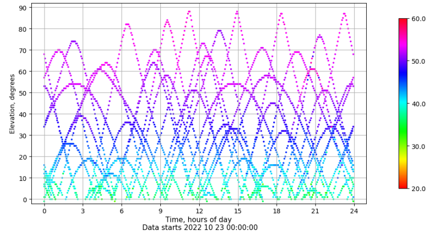
Time-elevation plot for station IZAN. Signal to Noise S1C Data file IZAN00ESP_R_2022296.xtr
