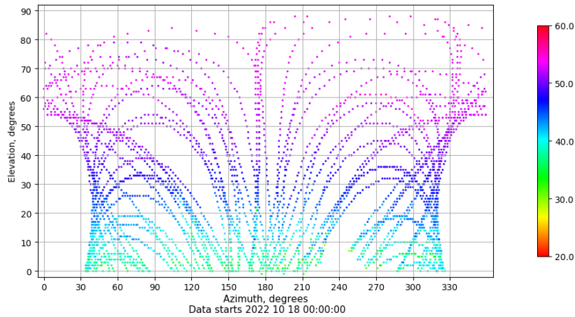
Azimuth-elevation plot for station IZAN. Signal to Noise S1C Data file IZAN00ESP_R_2022291.xtr
