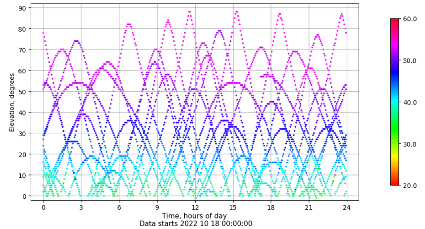
Time-elevation plot for station IZAN. Signal to Noise S1C Data file IZAN00ESP_R_2022291.xtr
