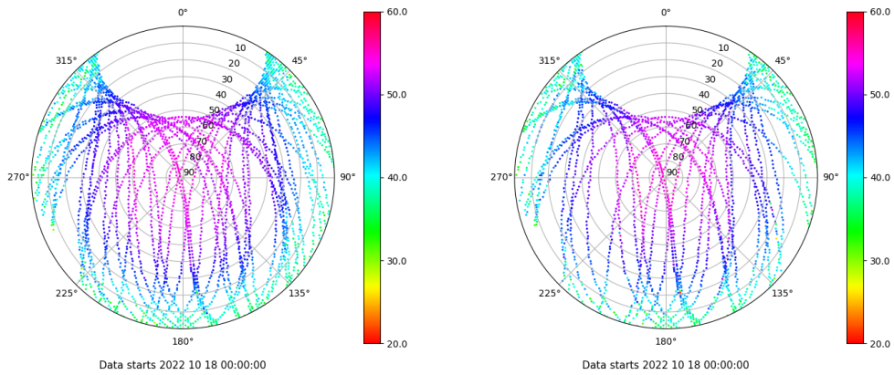
Skyplot for station IZAN. Signal to Noise S1C Data file IZAN00ESP_R_2022291.xtr Skyplot for station IZAN. Signal to Noise S2S Data file IZAN00ESP_R_2022291.xtr
