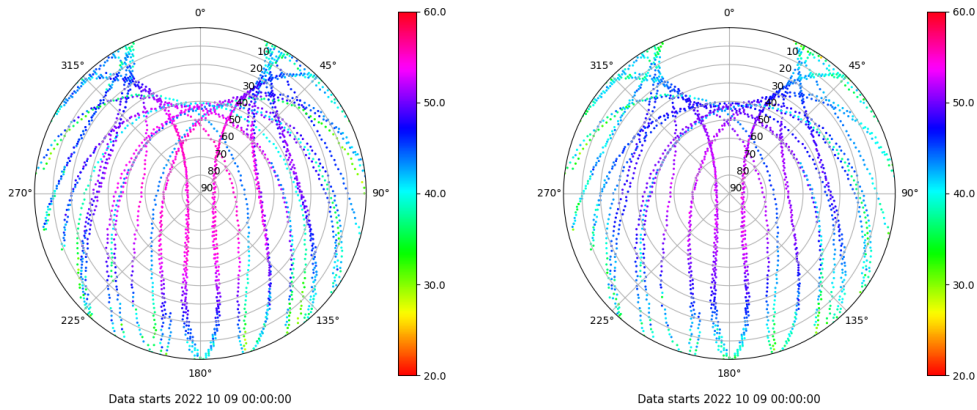
Skyplot for station IZAN. Signal to Noise S1C Data file IZAN00ESP_R_2022282.xtr Skyplot for station IZAN. Signal to Noise S2C Data file IZAN00ESP_R_2022282.xtr
