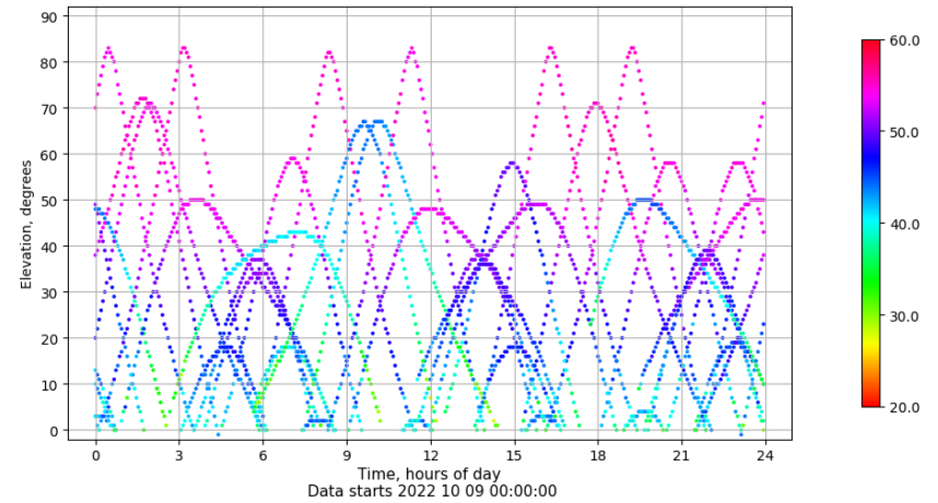
Time-elevation plot for station IZAN. Signal to Noise S1C Data file IZAN00ESP_R_2022282.xtr
