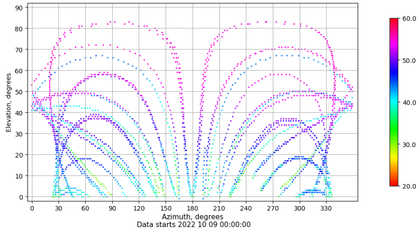
Azimuth-elevation plot for station IZAN. Signal to Noise S1C Data file IZAN00ESP_R_2022282.xtr
