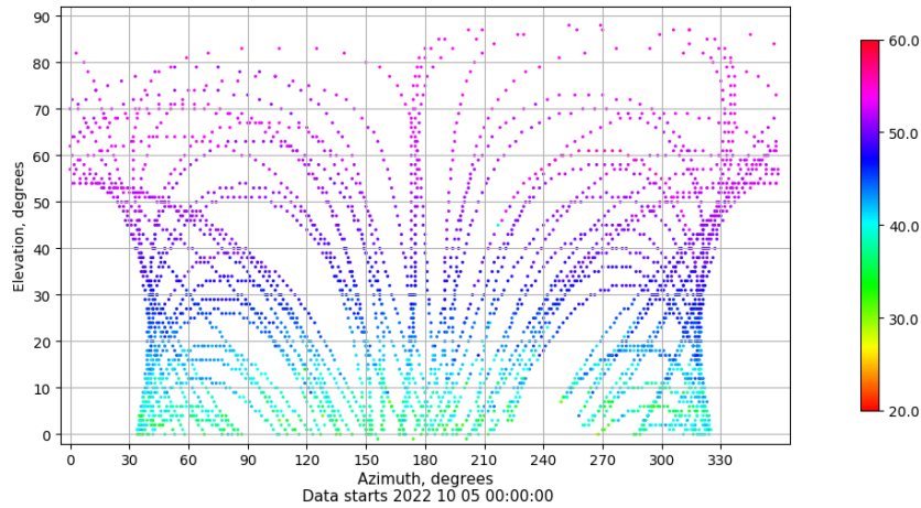
Azimuth-elevation plot for station IZAN. Signal to Noise S1C Data file IZAN00ESP_R_2022278.xtr
