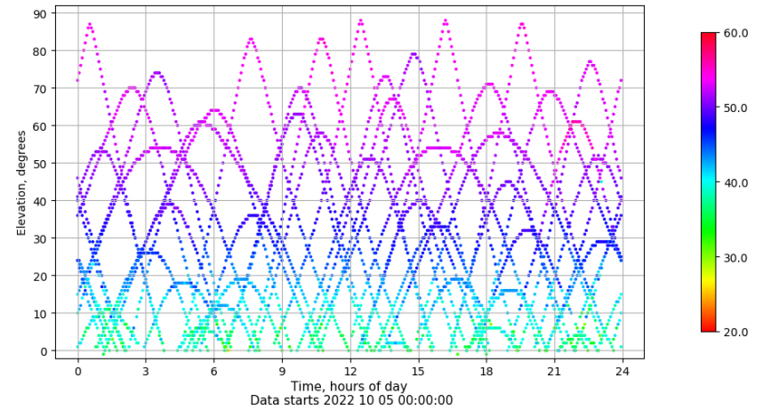
Time-elevation plot for station IZAN. Signal to Noise S1C Data file IZAN00ESP_R_2022278.xtr
