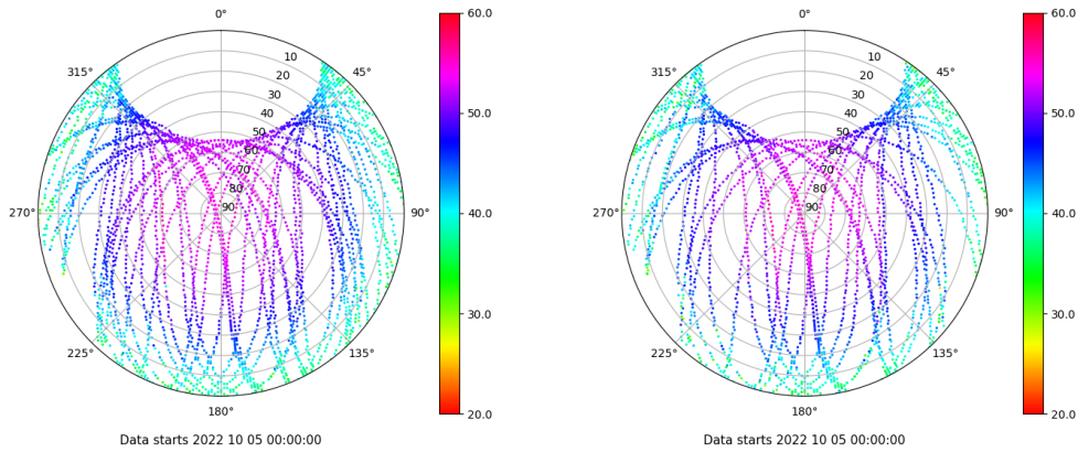
Skyplot for station IZAN. Signal to Noise S1C Data file IZAN00ESP_R_2022278.xtr Skyplot for station IZAN. Signal to Noise S2S Data file IZAN00ESP_R_2022278.xtr
