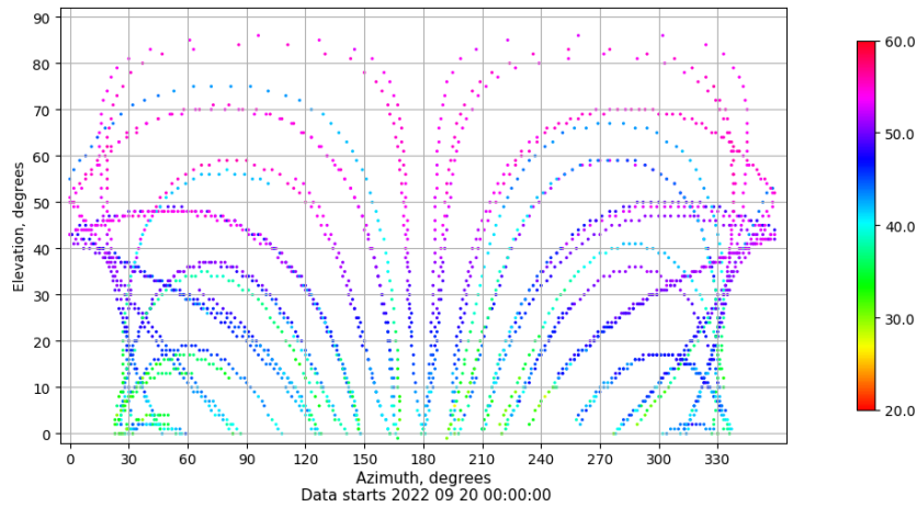
Azimuth-elevation plot for station IZAN. Signal to Noise S1C Data file IZAN00ESP_R_2022263.xtr
