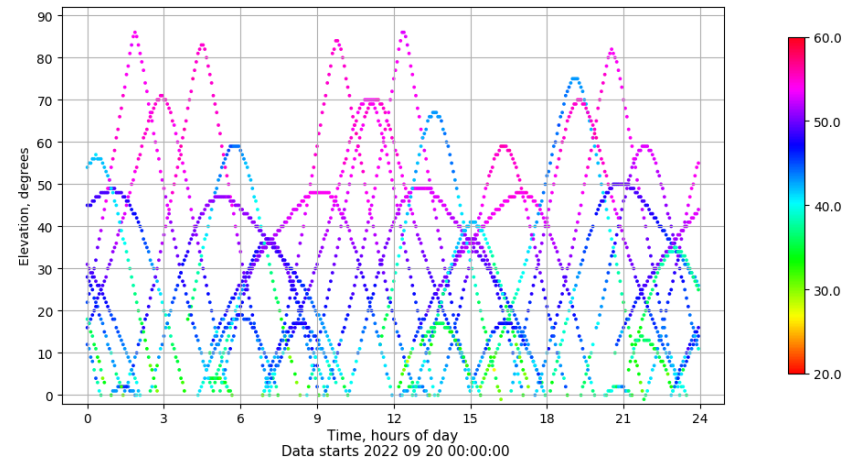
Time-elevation plot for station IZAN. Signal to Noise S1C Data file IZAN00ESP_R_2022263.xtr
