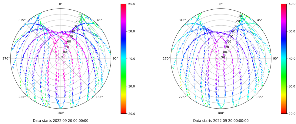
Skyplot for station IZAN. Signal to Noise S1C Data file IZAN00ESP_R_2022263.xtr Skyplot for station IZAN. Signal to Noise S2C Data file IZAN00ESP_R_2022263.xtr
