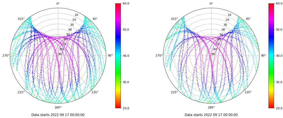
Skyplot for station IZAN. Signal to Noise S1C Data file IZAN00ESP_R_2022260.xtr Skyplot for station IZAN. Signal to Noise S2S Data file IZAN00ESP_R_2022260.xtr
