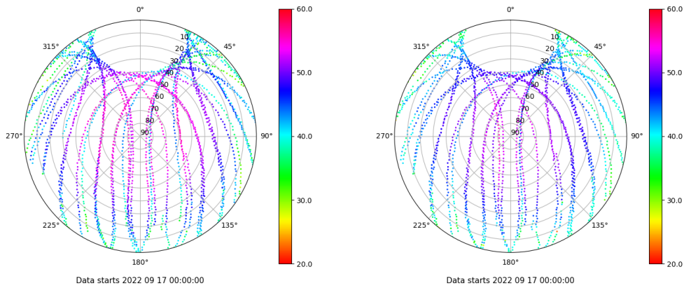
Skyplot for station IZAN. Signal to Noise S1C Data file IZAN00ESP_R_2022260.xtr Skyplot for station IZAN. Signal to Noise S2C Data file IZAN00ESP_R_2022260.xtr
