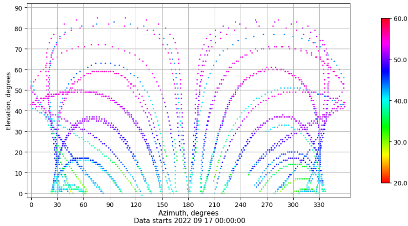
Azimuth-elevation plot for station IZAN. Signal to Noise S1C Data file IZAN00ESP_R_2022260.xtr
