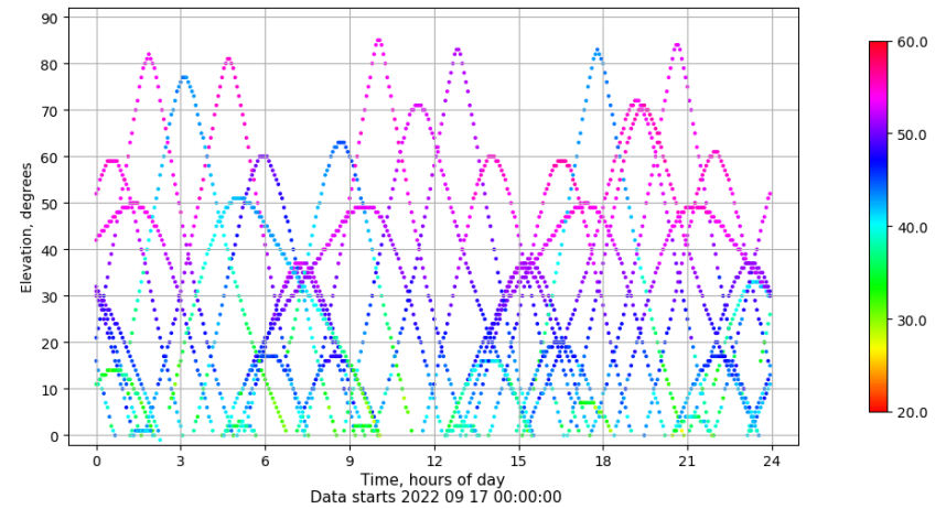
Time-elevation plot for station IZAN. Signal to Noise S1C Data file IZAN00ESP_R_2022260.xtr
