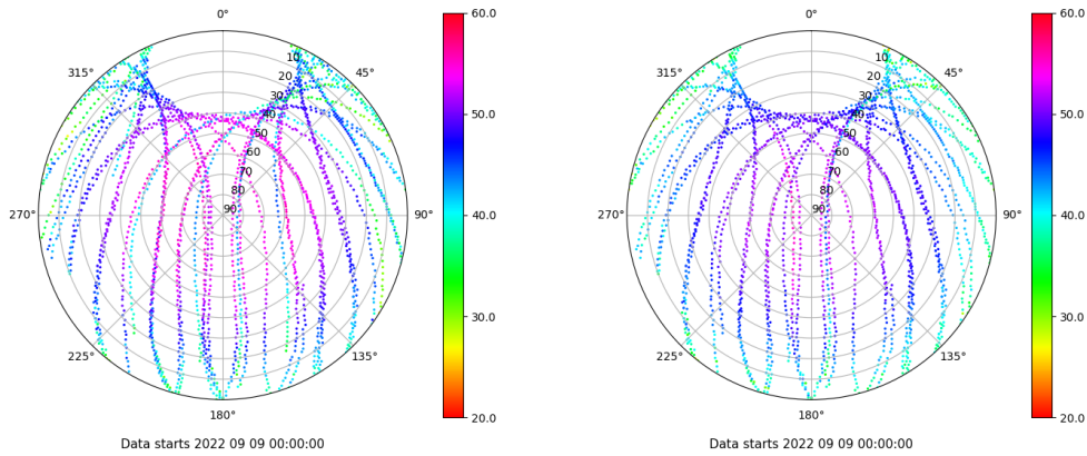
Skyplot for station IZAN. Signal to Noise S1C Data file IZAN00ESP_R_2022252.xtr Skyplot for station IZAN. Signal to Noise S2C Data file IZAN00ESP_R_2022252.xtr
