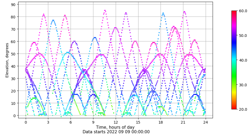
Time-elevation plot for station IZAN. Signal to Noise S1C Data file IZAN00ESP_R_2022252.xtr
