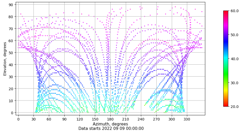
Azimuth-elevation plot for station IZAN. Signal to Noise S1C Data file IZAN00ESP_R_2022252.xtr
