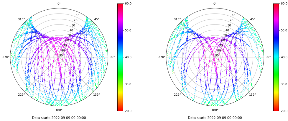
Skyplot for station IZAN. Signal to Noise S1C Data file IZAN00ESP_R_2022252.xtr Skyplot for station IZAN. Signal to Noise S2S Data file IZAN00ESP_R_2022252.xtr
