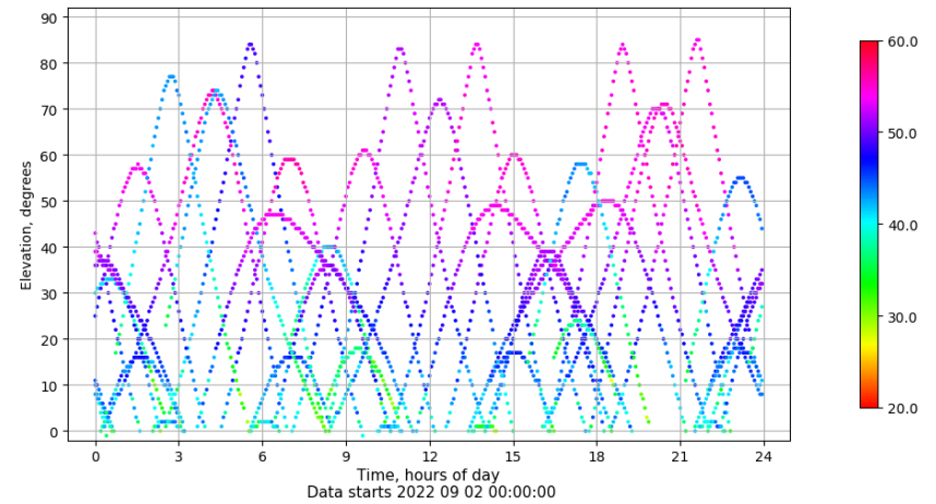
Time-elevation plot for station IZAN. Signal to Noise S1C Data file IZAN00ESP_R_2022245.xtr
