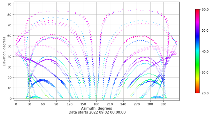
Azimuth-elevation plot for station IZAN. Signal to Noise S1C Data file IZAN00ESP_R_2022245.xtr
