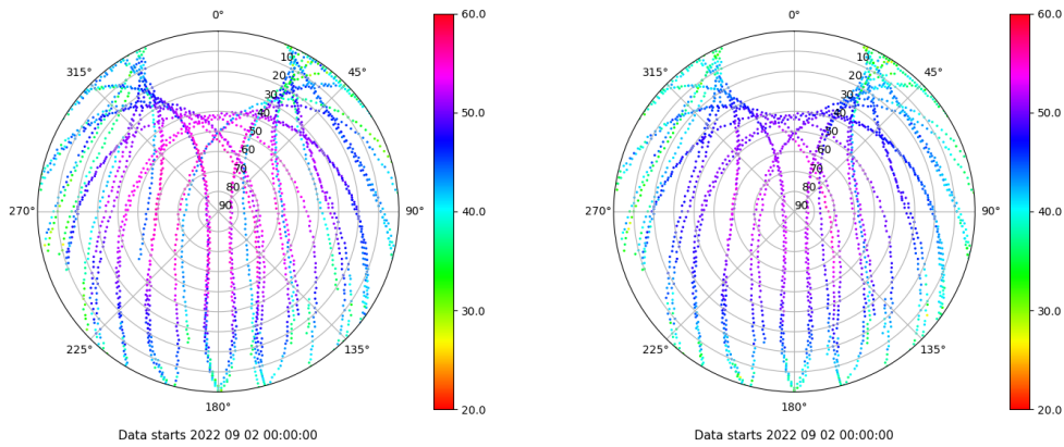
Skyplot for station IZAN. Signal to Noise S1C Data file IZAN00ESP_R_2022245.xtr Skyplot for station IZAN. Signal to Noise S2C Data file IZAN00ESP_R_2022245.xtr
