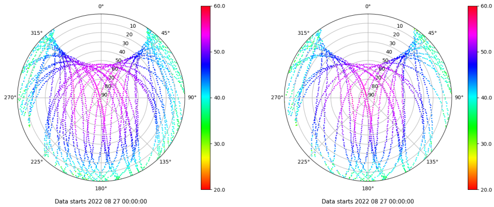
Skyplot for station IZAN. Signal to Noise S1C Data file IZAN00ESP_R_2022239.xtr Skyplot for station IZAN. Signal to Noise S2S Data file IZAN00ESP_R_2022239.xtr
