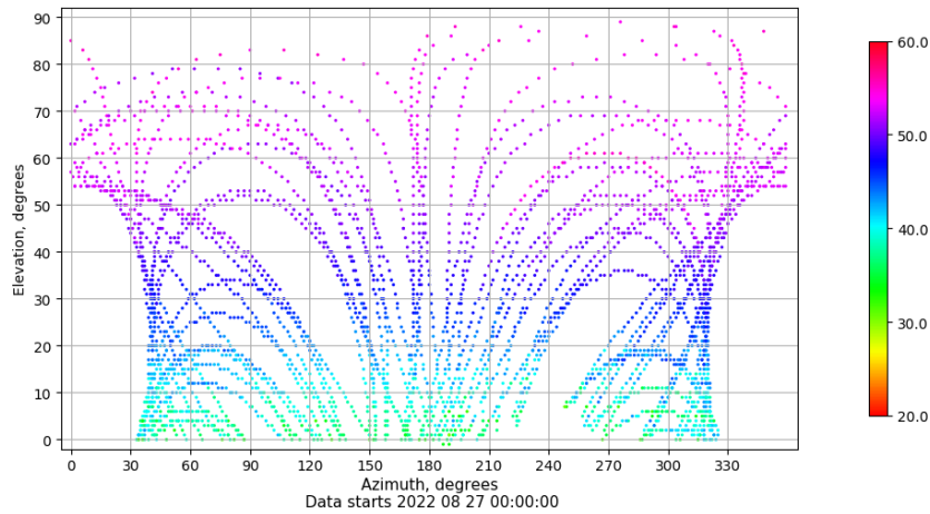
Azimuth-elevation plot for station IZAN. Signal to Noise S1C Data file IZAN00ESP_R_2022239.xtr
