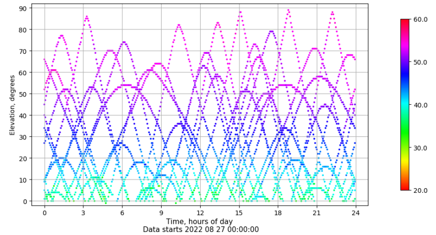
Time-elevation plot for station IZAN. Signal to Noise S1C Data file IZAN00ESP_R_2022239.xtr
