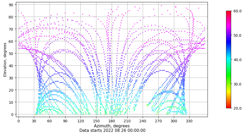
Azimuth-elevation plot for station IZAN. Signal to Noise S1C Data file IZAN00ESP_R_2022238.xtr
