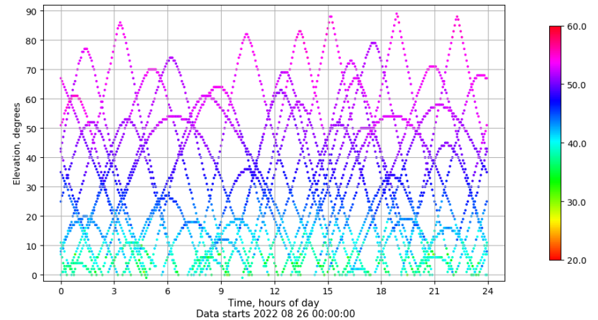
Time-elevation plot for station IZAN. Signal to Noise S1C Data file IZAN00ESP_R_2022238.xtr
