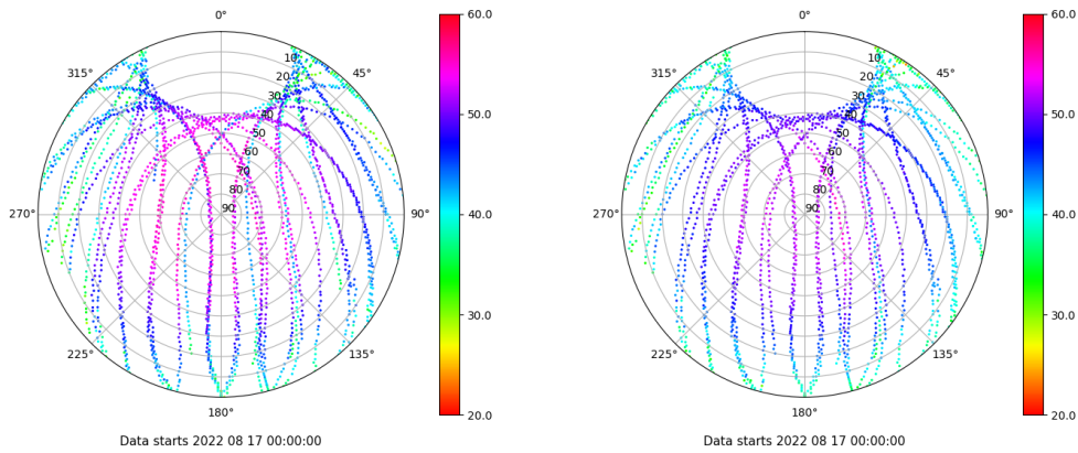
Skyplot for station IZAN. Signal to Noise S1C Data file IZAN00ESP_R_2022229.xtr Skyplot for station IZAN. Signal to Noise S2C Data file IZAN00ESP_R_2022229.xtr
