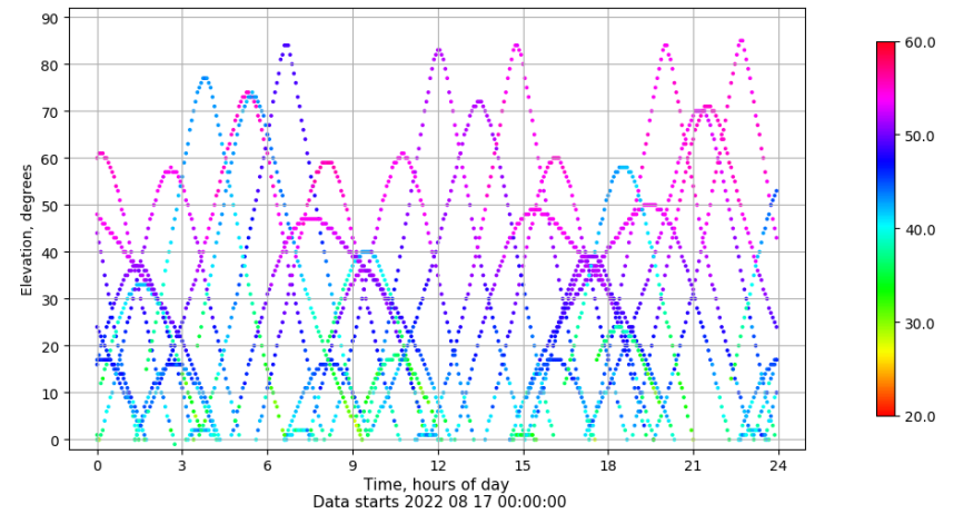
Time-elevation plot for station IZAN. Signal to Noise S1C Data file IZAN00ESP_R_2022229.xtr
