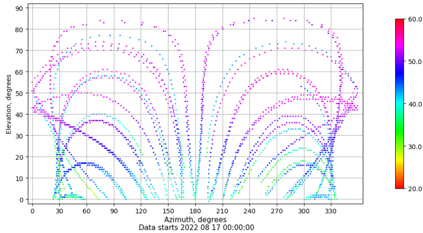
Azimuth-elevation plot for station IZAN. Signal to Noise S1C Data file IZAN00ESP_R_2022229.xtr
