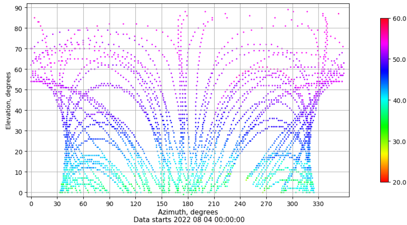
Azimuth-elevation plot for station IZAN. Signal to Noise S1C Data file IZAN00ESP_R_2022216.xtr
