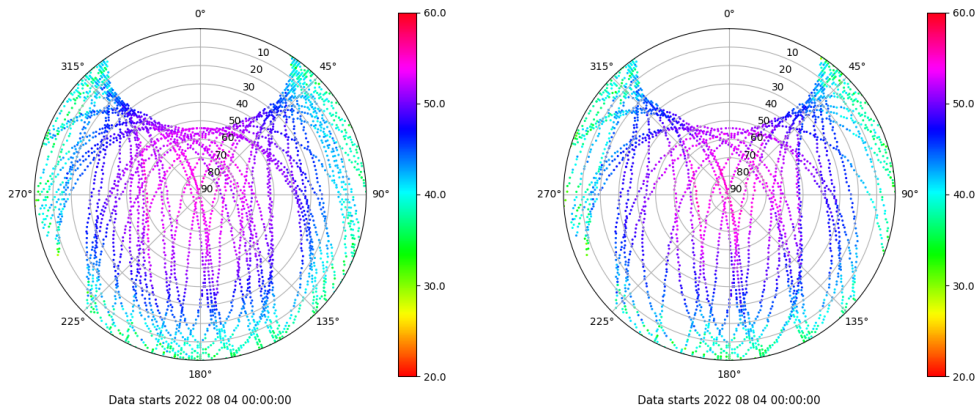
Skyplot for station IZAN. Signal to Noise S1C Data file IZAN00ESP_R_2022216.xtr Skyplot for station IZAN. Signal to Noise S2S Data file IZAN00ESP_R_2022216.xtr
