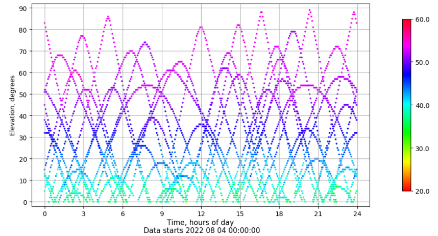
Time-elevation plot for station IZAN. Signal to Noise S1C Data file IZAN00ESP_R_2022216.xtr
