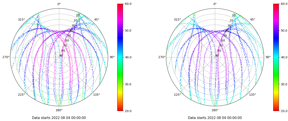
Skyplot for station IZAN. Signal to Noise S1C Data file IZAN00ESP_R_2022216.xtr Skyplot for station IZAN. Signal to Noise S2C Data file IZAN00ESP_R_2022216.xtr
