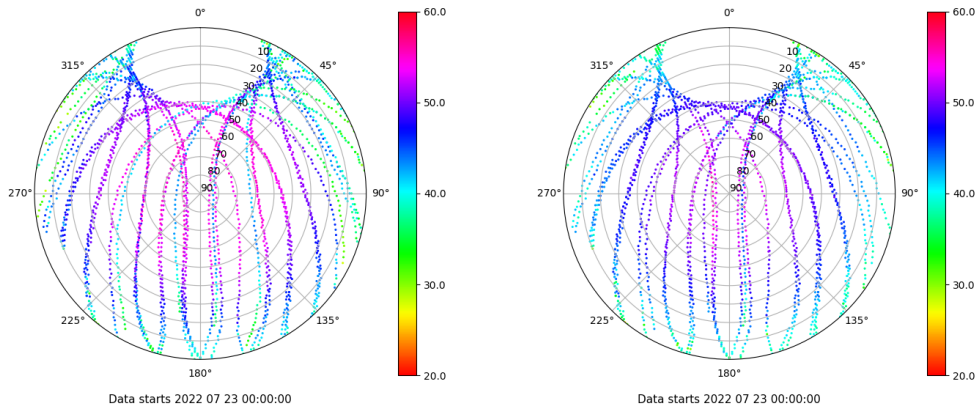
Skyplot for station IZAN. Signal to Noise S1C Data file IZAN00ESP_R_2022204.xtr Skyplot for station IZAN. Signal to Noise S2C Data file IZAN00ESP_R_2022204.xtr
