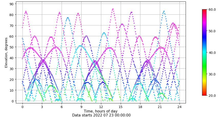
Time-elevation plot for station IZAN. Signal to Noise S1C Data file IZAN00ESP_R_2022204.xtr
