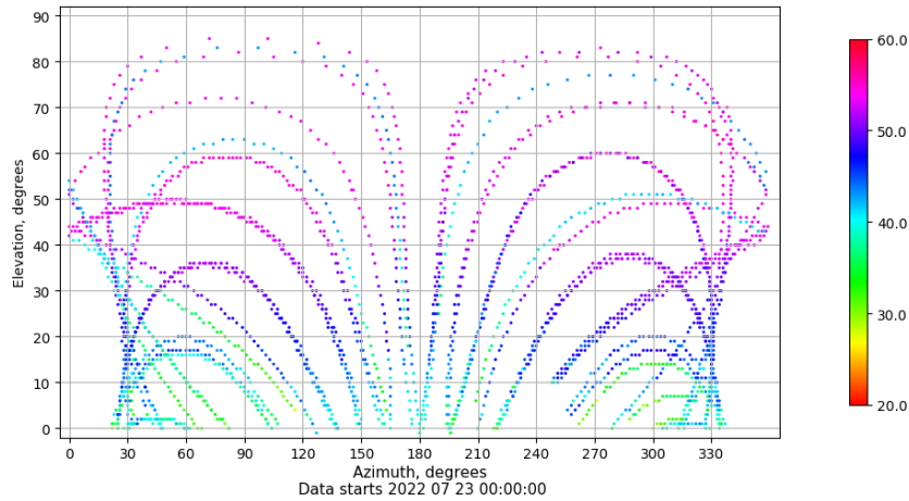
Azimuth-elevation plot for station IZAN. Signal to Noise S1C Data file IZAN00ESP_R_2022204.xtr
