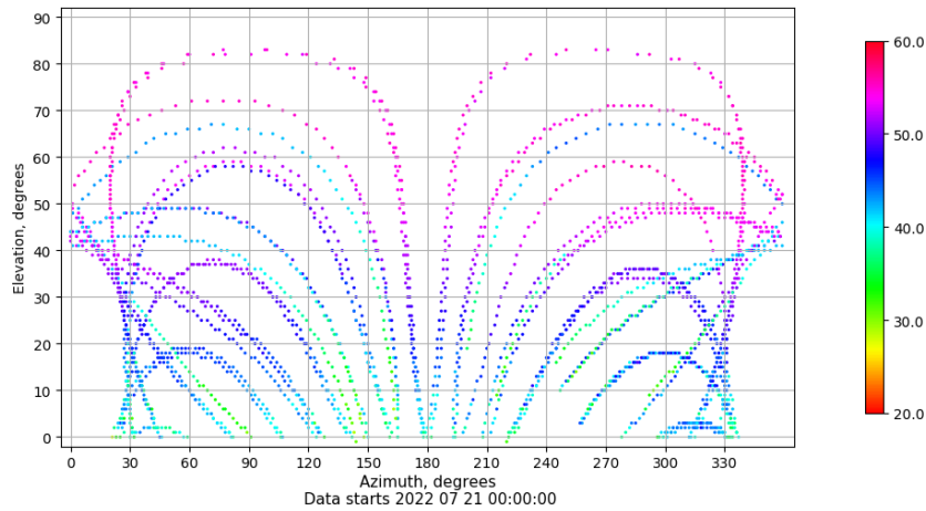
Azimuth-elevation plot for station IZAN. Signal to Noise S1C Data file IZAN00ESP_R_2022202.xtr
