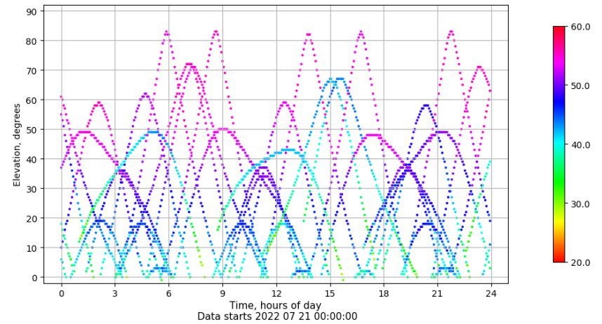
Time-elevation plot for station IZAN. Signal to Noise S1C Data file IZAN00ESP_R_2022202.xtr
