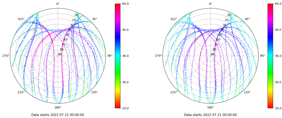
Skyplot for station IZAN. Signal to Noise S1C Data file IZAN00ESP_R_2022202.xtr Skyplot for station IZAN. Signal to Noise S2C Data file IZAN00ESP_R_2022202.xtr
