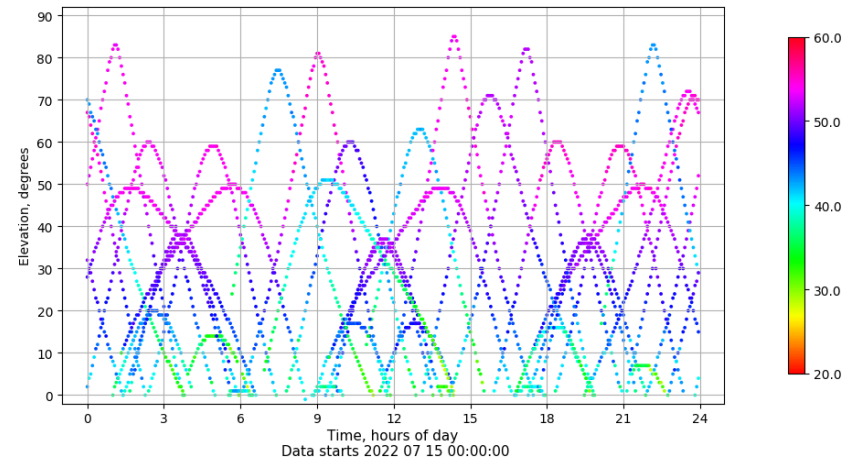
Time-elevation plot for station IZAN. Signal to Noise S1C Data file IZAN00ESP_R_2022196.xtr
