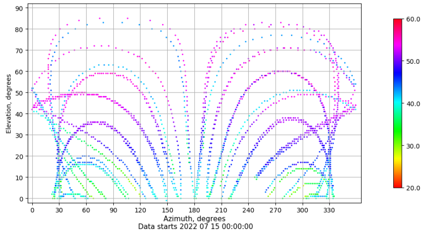
Azimuth-elevation plot for station IZAN. Signal to Noise S1C Data file IZAN00ESP_R_2022196.xtr
