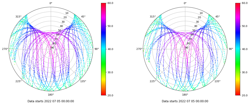
Skyplot for station IZAN. Signal to Noise S1C Data file IZAN00ESP_R_2022186.xtr Skyplot for station IZAN. Signal to Noise S2S Data file IZAN00ESP_R_2022186.xtr
