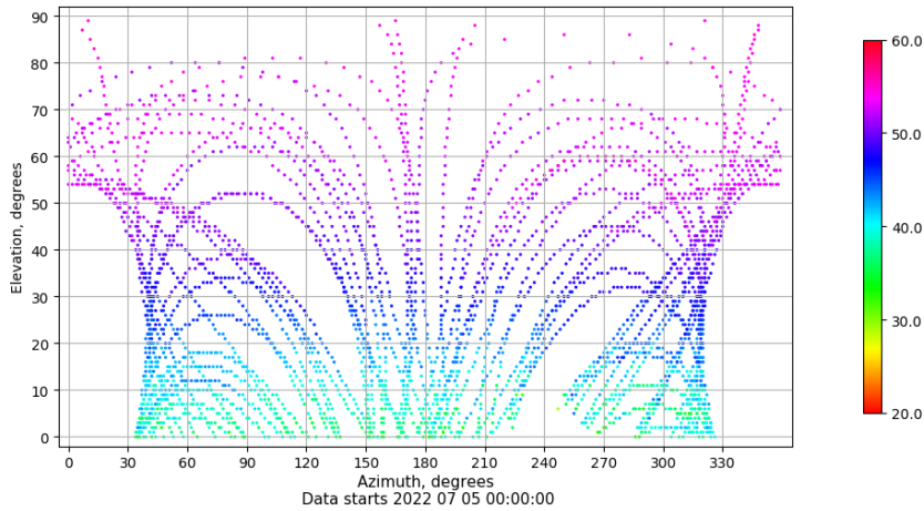
Azimuth-elevation plot for station IZAN. Signal to Noise S1C Data file IZAN00ESP_R_2022186.xtr
