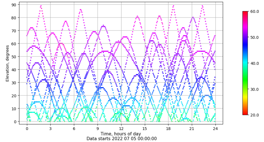
Time-elevation plot for station IZAN. Signal to Noise S1C Data file IZAN00ESP_R_2022186.xtr
