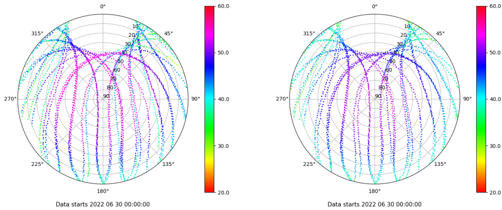
Skyplot for station IZAN. Signal to Noise S1C Data file IZAN00ESP_R_2022181.xtr Skyplot for station IZAN. Signal to Noise S2C Data file IZAN00ESP_R_2022181.xtr
