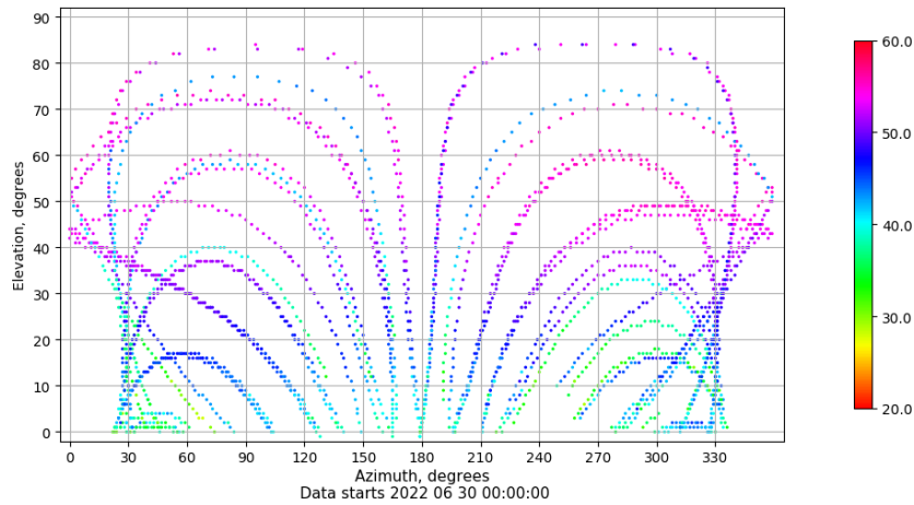
Azimuth-elevation plot for station IZAN. Signal to Noise S1C Data file IZAN00ESP_R_2022181.xtr
