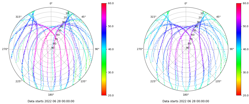
Skyplot for station IZAN. Signal to Noise S1C Data file IZAN00ESP_R_2022179.xtr Skyplot for station IZAN. Signal to Noise S2C Data file IZAN00ESP_R_2022179.xtr
