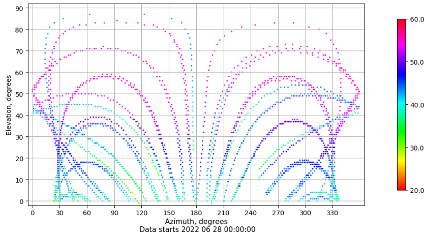
Azimuth-elevation plot for station IZAN. Signal to Noise S1C Data file IZAN00ESP_R_2022179.xtr
