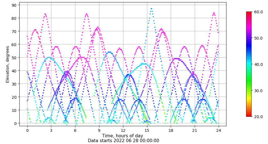
Time-elevation plot for station IZAN. Signal to Noise S1C Data file IZAN00ESP_R_2022179.xtr
