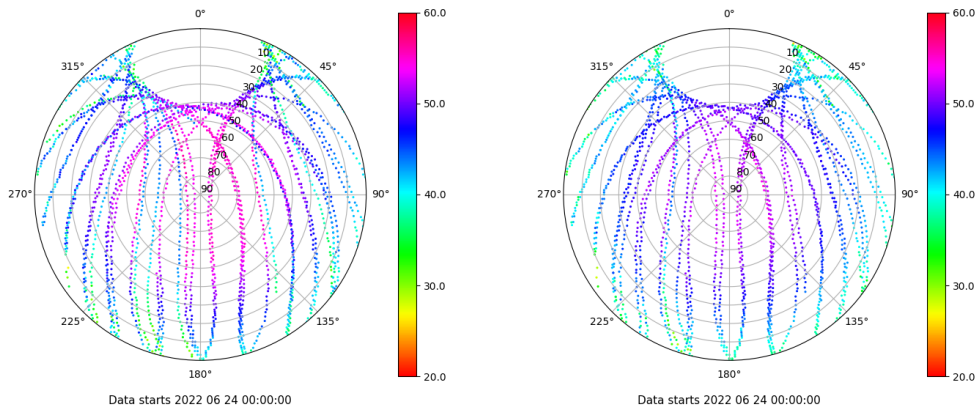
Skyplot for station IZAN. Signal to Noise S1C Data file IZAN00ESP_R_2022175.xtr Skyplot for station IZAN. Signal to Noise S2C Data file IZAN00ESP_R_2022175.xtr
