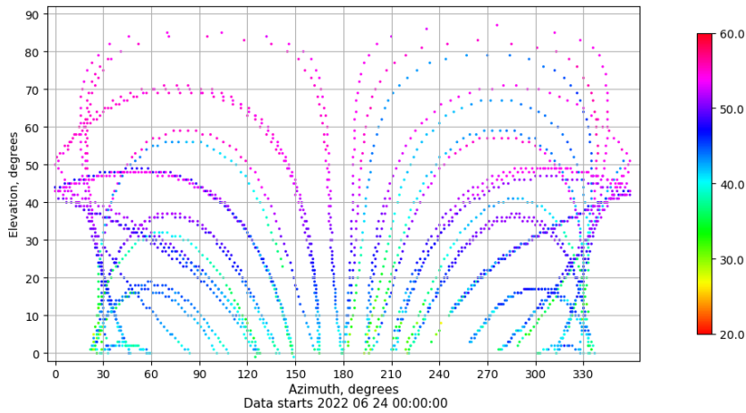
Azimuth-elevation plot for station IZAN. Signal to Noise S1C Data file IZAN00ESP_R_2022175.xtr
