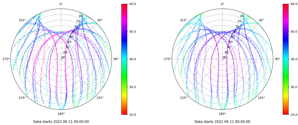
Skyplot for station IZAN. Signal to Noise S1C Data file IZAN00ESP_R_2022162.xtr Skyplot for station IZAN. Signal to Noise S2C Data file IZAN00ESP_R_2022162.xtr
