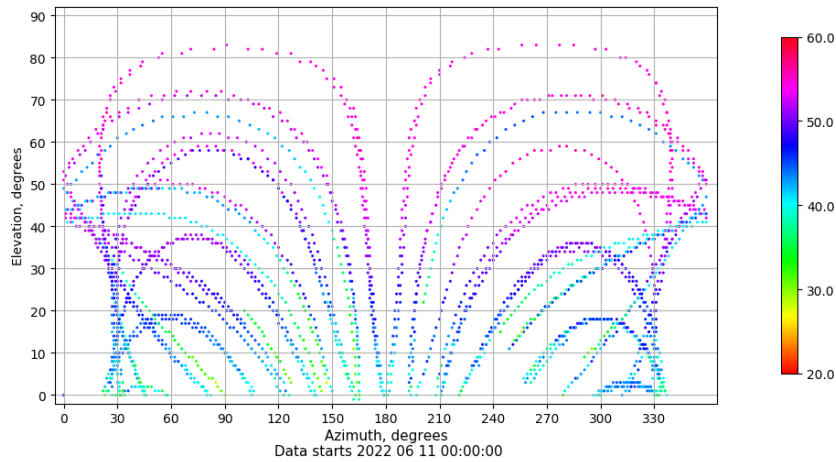
Azimuth-elevation plot for station IZAN. Signal to Noise S1C Data file IZAN00ESP_R_2022162.xtr
