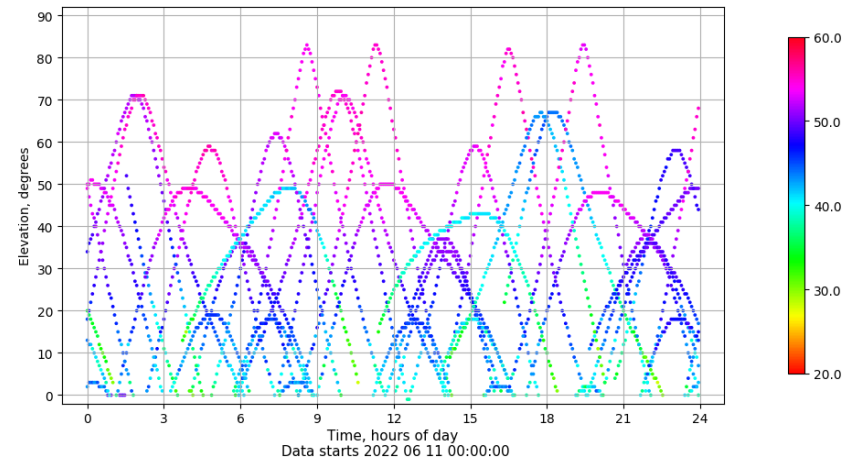
Time-elevation plot for station IZAN. Signal to Noise S1C Data file IZAN00ESP_R_2022162.xtr
