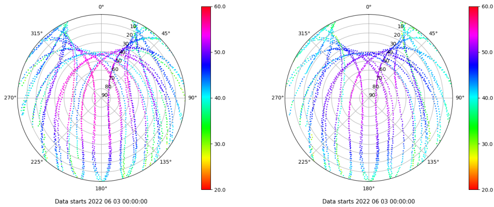
Skyplot for station IZAN. Signal to Noise S1C Data file IZAN00ESP_R_2022154.xtr Skyplot for station IZAN. Signal to Noise S2C Data file IZAN00ESP_R_2022154.xtr
