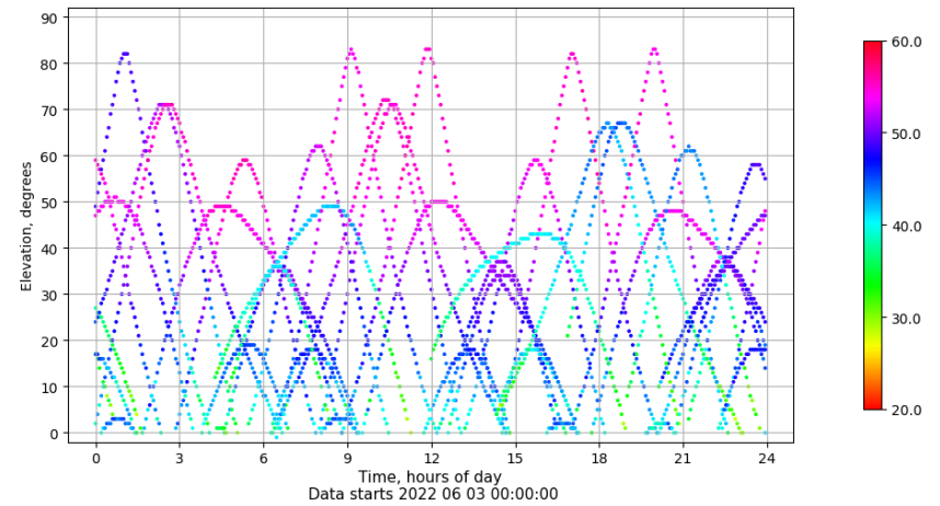
Time-elevation plot for station IZAN. Signal to Noise S1C Data file IZAN00ESP_R_2022154.xtr
