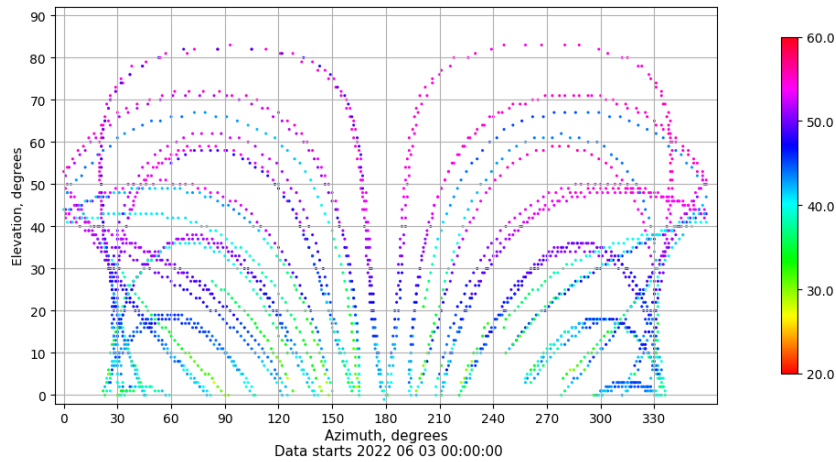
Azimuth-elevation plot for station IZAN. Signal to Noise S1C Data file IZAN00ESP_R_2022154.xtr
