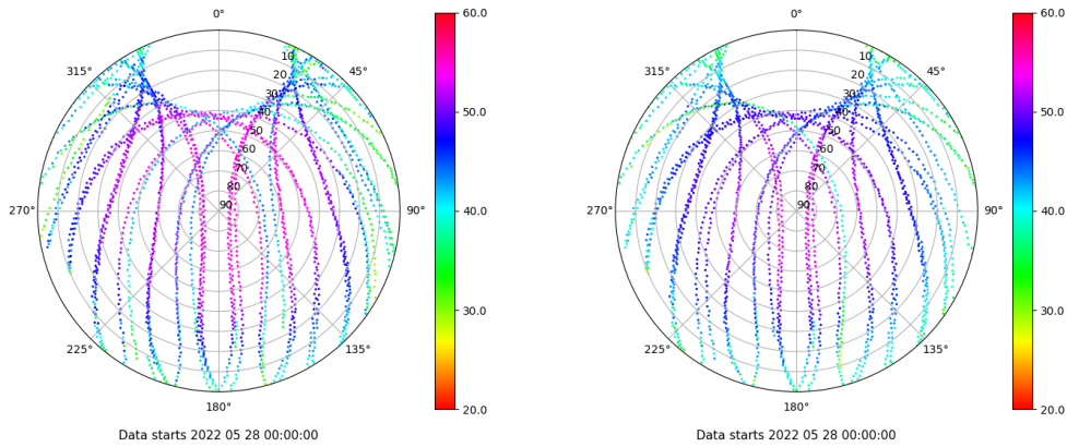
Skyplot for station IZAN. Signal to Noise S1C Data file IZAN00ESP_R_2022148.xtr Skyplot for station IZAN. Signal to Noise S2C Data file IZAN00ESP_R_2022148.xtr
