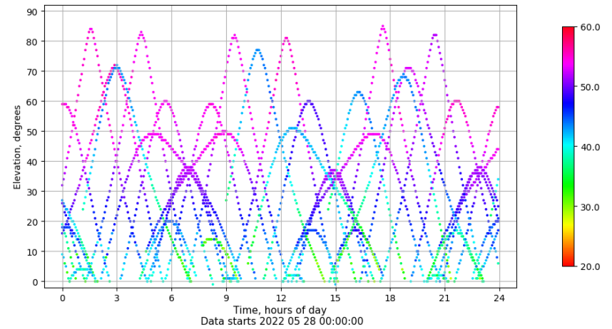
Time-elevation plot for station IZAN. Signal to Noise S1C Data file IZAN00ESP_R_2022148.xtr
