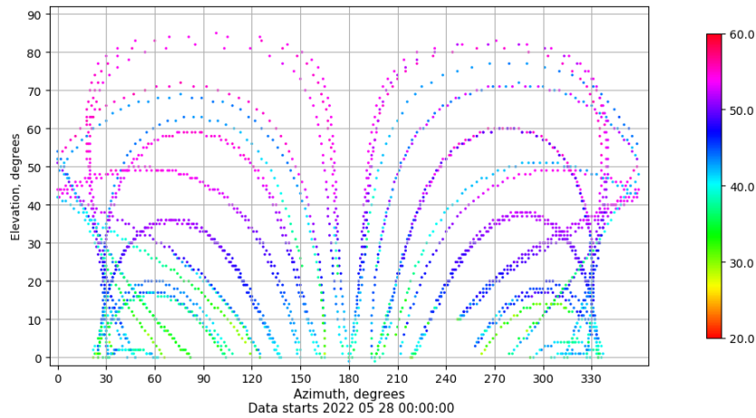
Azimuth-elevation plot for station IZAN. Signal to Noise S1C Data file IZAN00ESP_R_2022148.xtr
