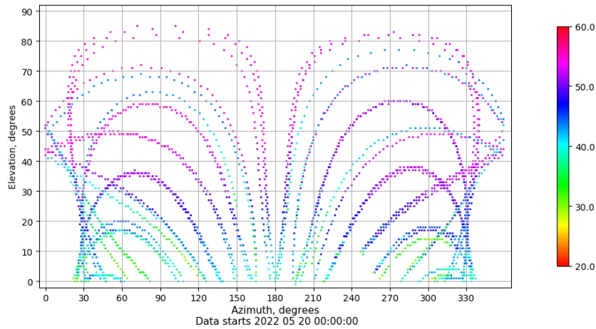
Azimuth-elevation plot for station IZAN. Signal to Noise S1C Data file IZAN00ESP_R_2022140.xtr
