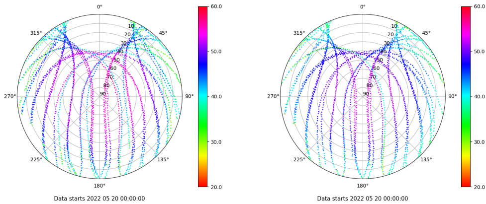
Skyplot for station IZAN. Signal to Noise S1C Data file IZAN00ESP_R_2022140.xtr Skyplot for station IZAN. Signal to Noise S2C Data file IZAN00ESP_R_2022140.xtr
