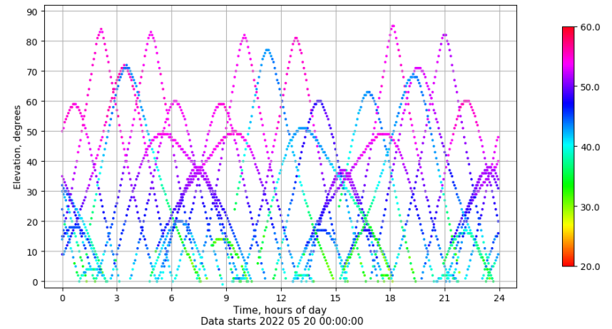
Time-elevation plot for station IZAN. Signal to Noise S1C Data file IZAN00ESP_R_2022140.xtr
