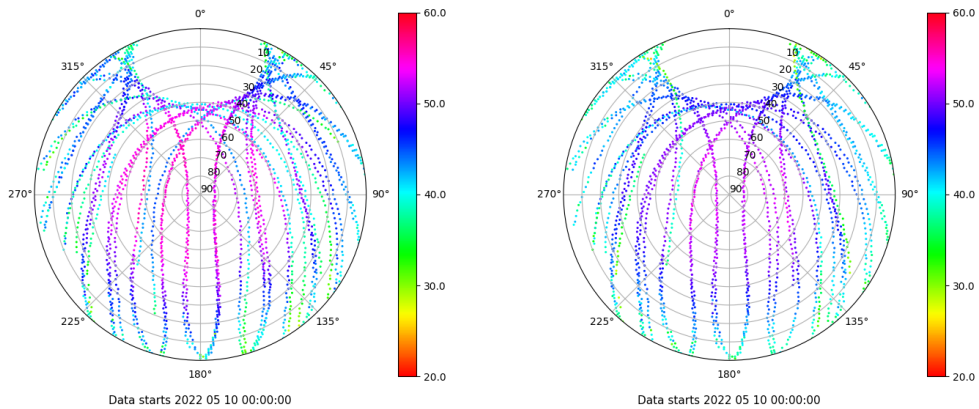
Skyplot for station IZAN. Signal to Noise S1C Data file IZAN00ESP_R_2022130.xtr Skyplot for station IZAN. Signal to Noise S2C Data file IZAN00ESP_R_2022130.xtr
