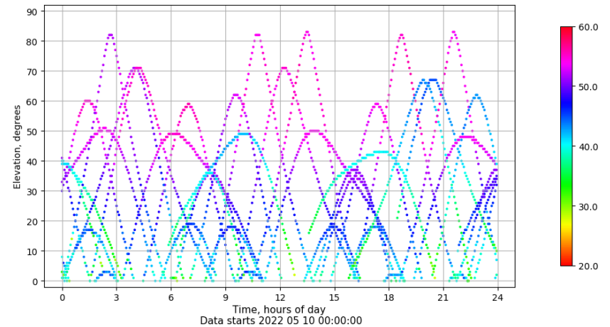
Time-elevation plot for station IZAN. Signal to Noise S1C Data file IZAN00ESP_R_2022130.xtr
