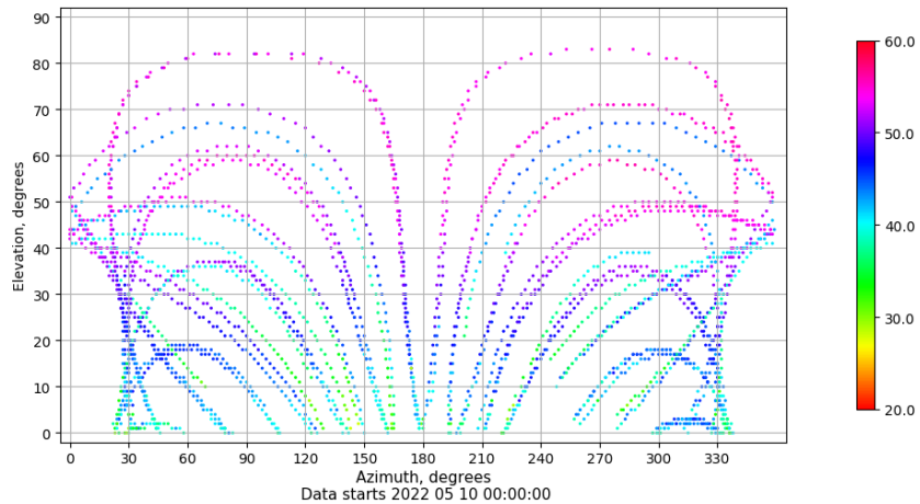
Azimuth-elevation plot for station IZAN. Signal to Noise S1C Data file IZAN00ESP_R_2022130.xtr
