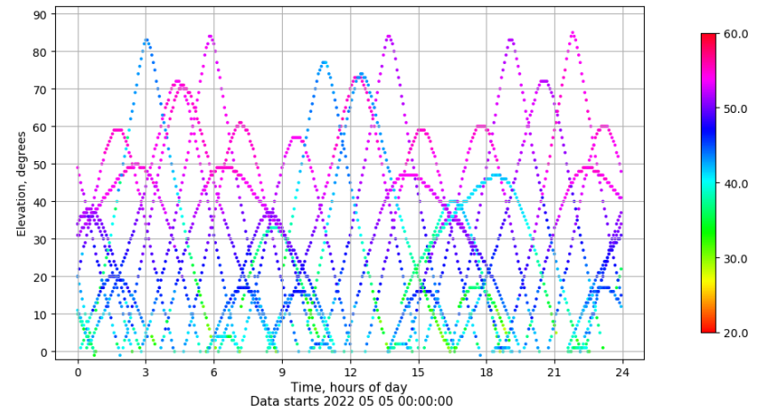
Time-elevation plot for station IZAN. Signal to Noise S1C Data file IZAN00ESP_R_2022125.xtr
