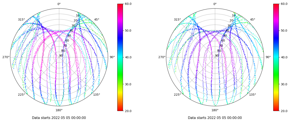
Skyplot for station IZAN. Signal to Noise S1C Data file IZAN00ESP_R_2022125.xtr Skyplot for station IZAN. Signal to Noise S2C Data file IZAN00ESP_R_2022125.xtr
