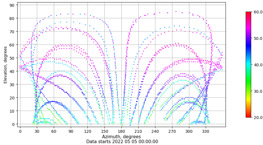
Azimuth-elevation plot for station IZAN. Signal to Noise S1C Data file IZAN00ESP_R_2022125.xtr
