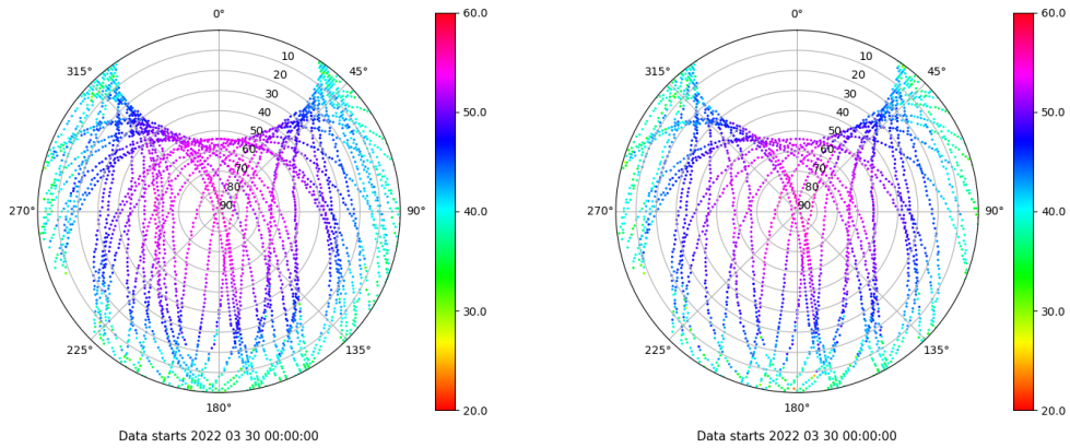
Skyplot for station IZAN. Signal to Noise S1C Data file IZAN00ESP_R_2022089.xtr Skyplot for station IZAN. Signal to Noise S2S Data file IZAN00ESP_R_2022089.xtr
