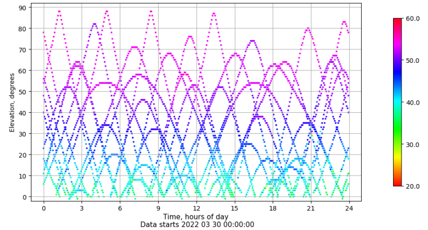
Time-elevation plot for station IZAN. Signal to Noise S1C Data file IZAN00ESP_R_2022089.xtr
