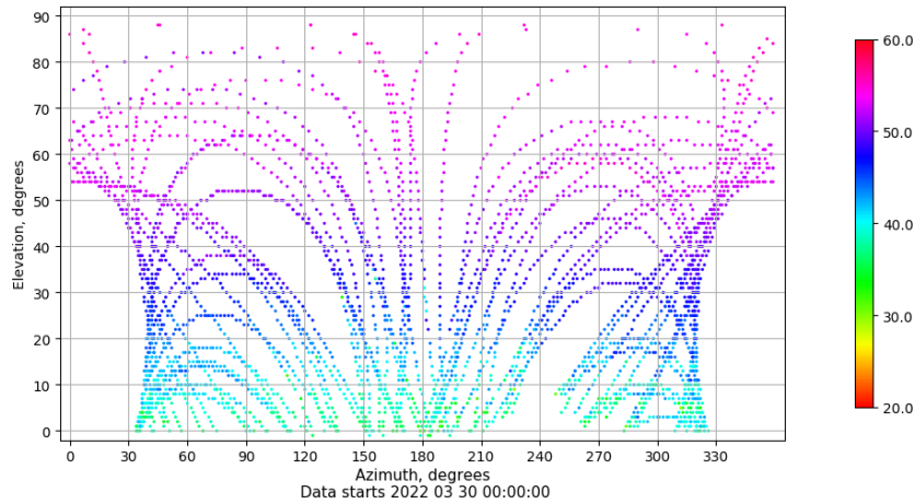
Azimuth-elevation plot for station IZAN. Signal to Noise S1C Data file IZAN00ESP_R_2022089.xtr
