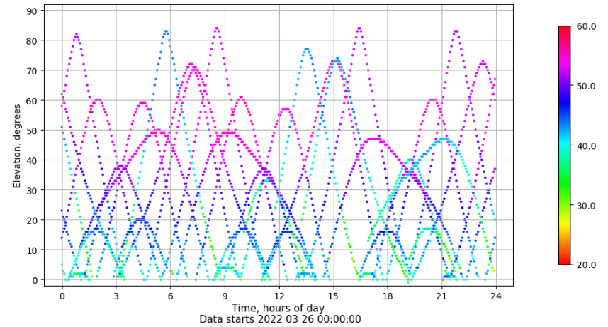
Time-elevation plot for station IZAN. Signal to Noise S1C Data file IZAN00ESP_R_2022085.xtr
