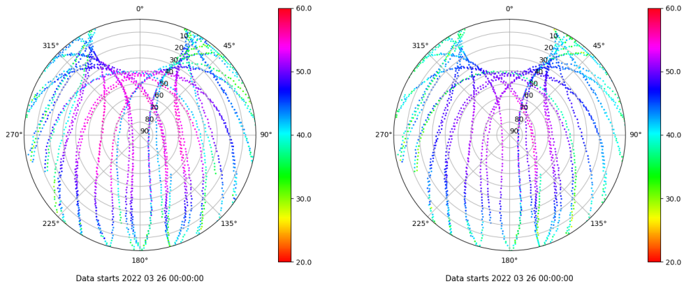
Skyplot for station IZAN. Signal to Noise S1C Data file IZAN00ESP_R_2022085.xtr Skyplot for station IZAN. Signal to Noise S2C Data file IZAN00ESP_R_2022085.xtr
