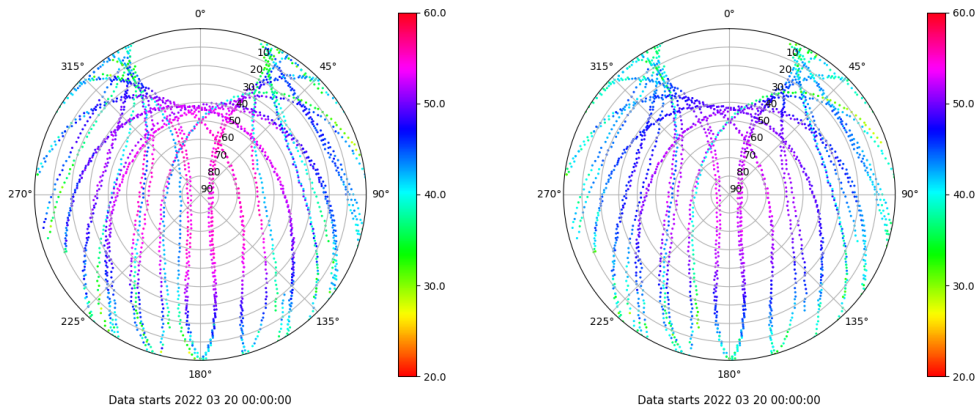
Skyplot for station IZAN. Signal to Noise S1C Data file IZAN00ESP_R_2022079.xtr Skyplot for station IZAN. Signal to Noise S2C Data file IZAN00ESP_R_2022079.xtr
