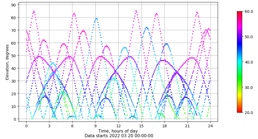
Time-elevation plot for station IZAN. Signal to Noise S1C Data file IZAN00ESP_R_2022079.xtr
