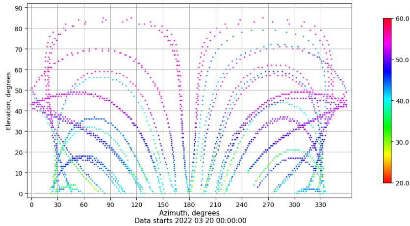
Azimuth-elevation plot for station IZAN. Signal to Noise S1C Data file IZAN00ESP_R_2022079.xtr
