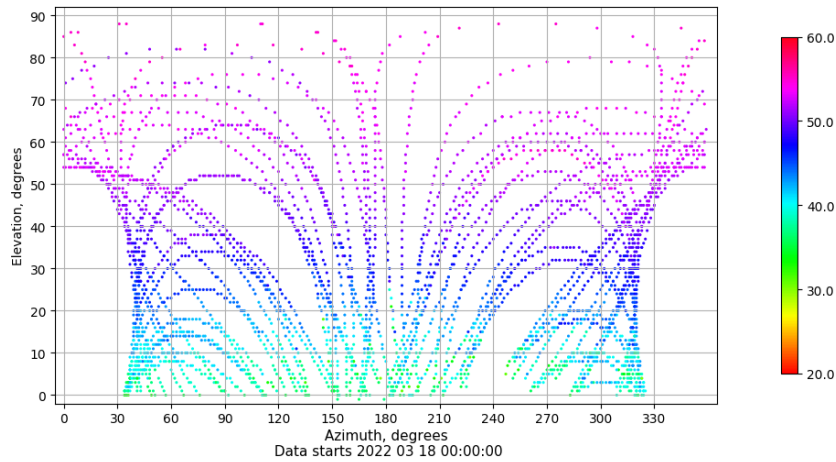
Azimuth-elevation plot for station IZAN. Signal to Noise S1C Data file IZAN00ESP_R_2022077.xtr
