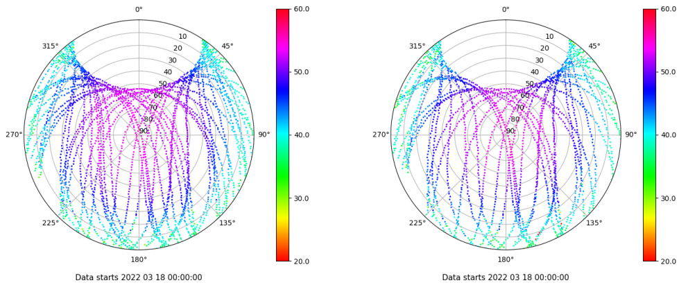
Skyplot for station IZAN. Signal to Noise S1C Data file IZAN00ESP_R_2022077.xtr Skyplot for station IZAN. Signal to Noise S2S Data file IZAN00ESP_R_2022077.xtr
