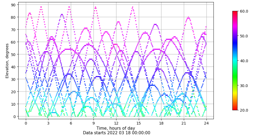
Time-elevation plot for station IZAN. Signal to Noise S1C Data file IZAN00ESP_R_2022077.xtr
