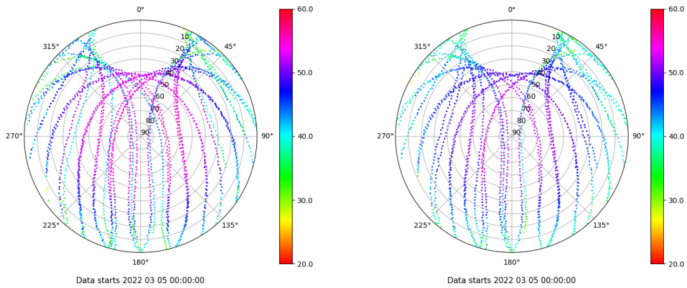
Skyplot for station IZAN. Signal to Noise S1C Data file IZAN00ESP_R_2022064.xtr Skyplot for station IZAN. Signal to Noise S2C Data file IZAN00ESP_R_2022064.xtr
