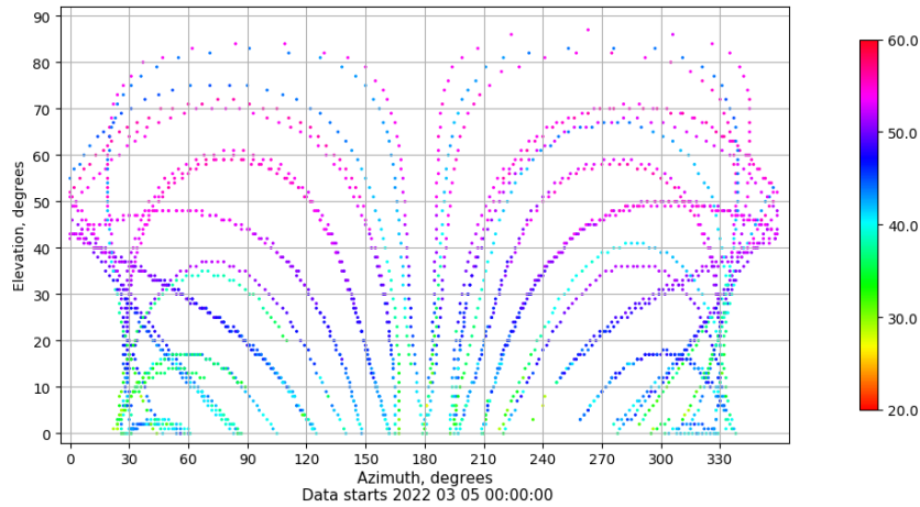
Azimuth-elevation plot for station IZAN. Signal to Noise S1C Data file IZAN00ESP_R_2022064.xtr
