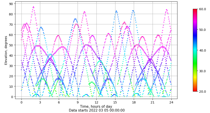
Time-elevation plot for station IZAN. Signal to Noise S1C Data file IZAN00ESP_R_2022064.xtr
