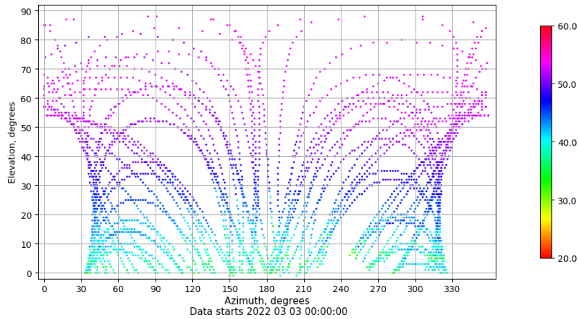
Azimuth-elevation plot for station IZAN. Signal to Noise S1C Data file IZAN00ESP_R_2022062.xtr
