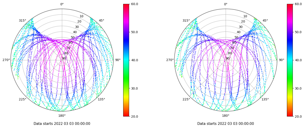
Skyplot for station IZAN. Signal to Noise S1C Data file IZAN00ESP_R_2022062.xtr Skyplot for station IZAN. Signal to Noise S2S Data file IZAN00ESP_R_2022062.xtr
