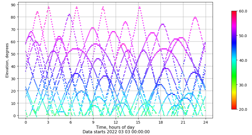
Time-elevation plot for station IZAN. Signal to Noise S1C Data file IZAN00ESP_R_2022062.xtr
