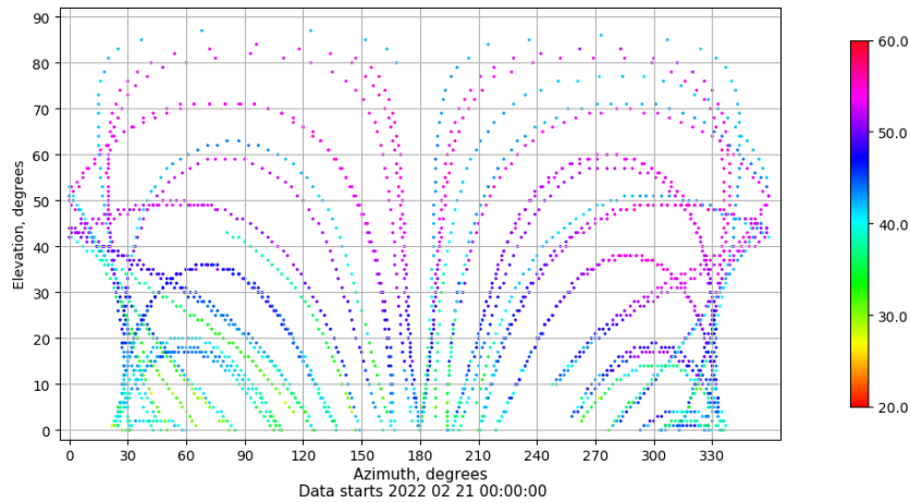
Azimuth-elevation plot for station IZAN. Signal to Noise S1C Data file IZAN00ESP_R_2022052.xtr
