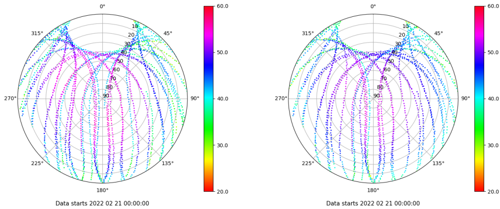
Skyplot for station IZAN. Signal to Noise S1C Data file IZAN00ESP_R_2022052.xtr Skyplot for station IZAN. Signal to Noise S2C Data file IZAN00ESP_R_2022052.xtr
