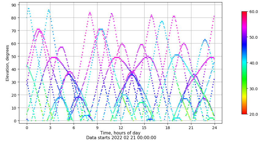
Time-elevation plot for station IZAN. Signal to Noise S1C Data file IZAN00ESP_R_2022052.xtr
