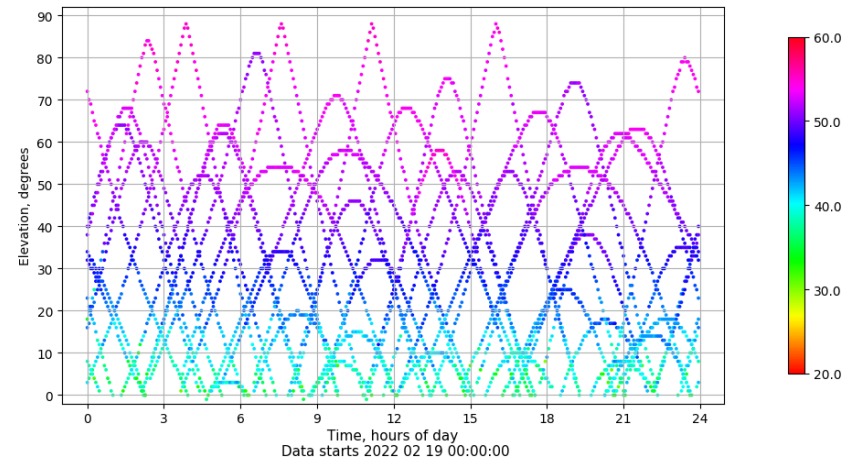
Time-elevation plot for station IZAN. Signal to Noise S1C Data file IZAN00ESP_R_2022050.xtr
