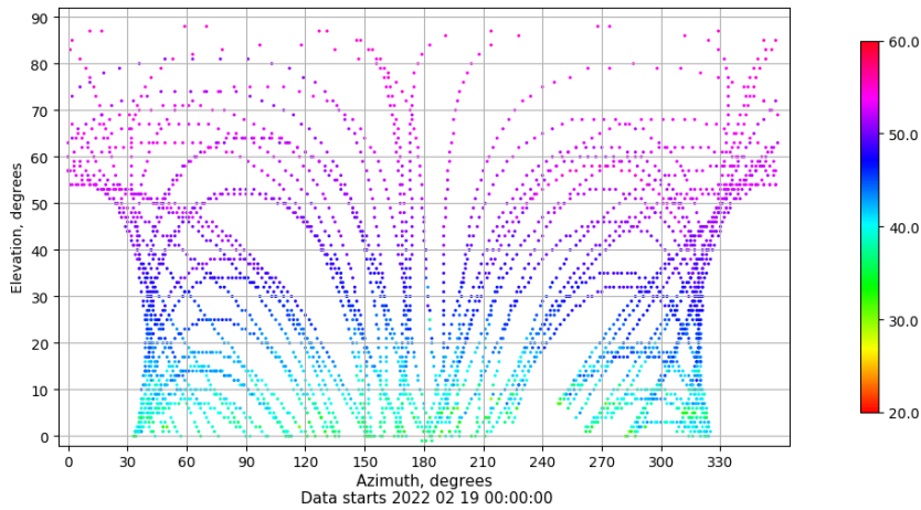
Azimuth-elevation plot for station IZAN. Signal to Noise S1C Data file IZAN00ESP_R_2022050.xtr
