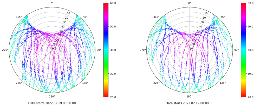
Skyplot for station IZAN. Signal to Noise S1C Data file IZAN00ESP_R_2022050.xtr Skyplot for station IZAN. Signal to Noise S2S Data file IZAN00ESP_R_2022050.xtr
