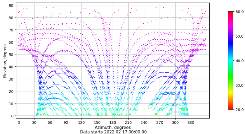
Azimuth-elevation plot for station IZAN. Signal to Noise S1C Data file IZAN00ESP_R_2022048.xtr
