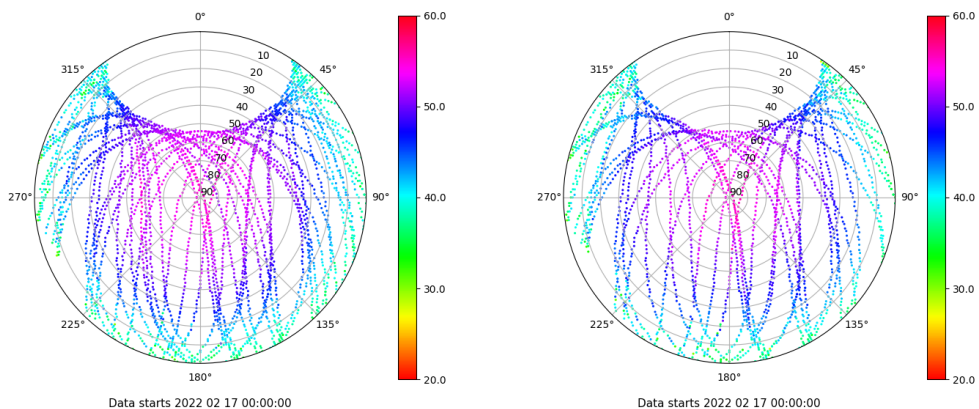
Skyplot for station IZAN. Signal to Noise S1C Data file IZAN00ESP_R_2022048.xtr Skyplot for station IZAN. Signal to Noise S2S Data file IZAN00ESP_R_2022048.xtr
