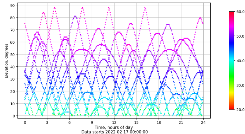
Time-elevation plot for station IZAN. Signal to Noise S1C Data file IZAN00ESP_R_2022048.xtr
