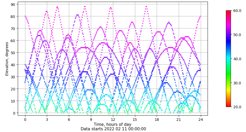
Time-elevation plot for station IZAN. Signal to Noise S1C Data file IZAN00ESP_R_2022042.xtr
