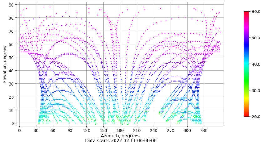
Azimuth-elevation plot for station IZAN. Signal to Noise S1C Data file IZAN00ESP_R_2022042.xtr
