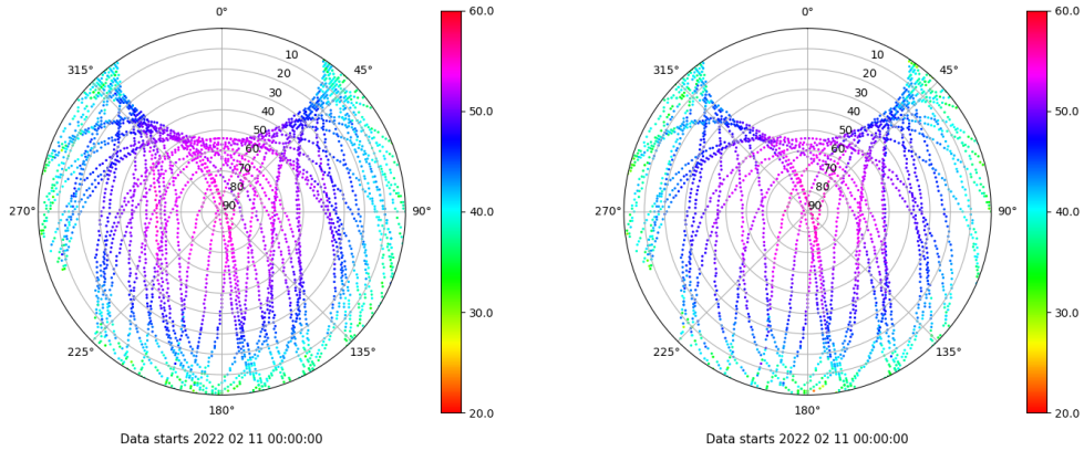
Skyplot for station IZAN. Signal to Noise S1C Data file IZAN00ESP_R_2022042.xtr Skyplot for station IZAN. Signal to Noise S2S Data file IZAN00ESP_R_2022042.xtr
