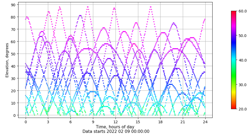
Time-elevation plot for station IZAN. Signal to Noise S1C Data file IZAN00ESP_R_2022040.xtr
