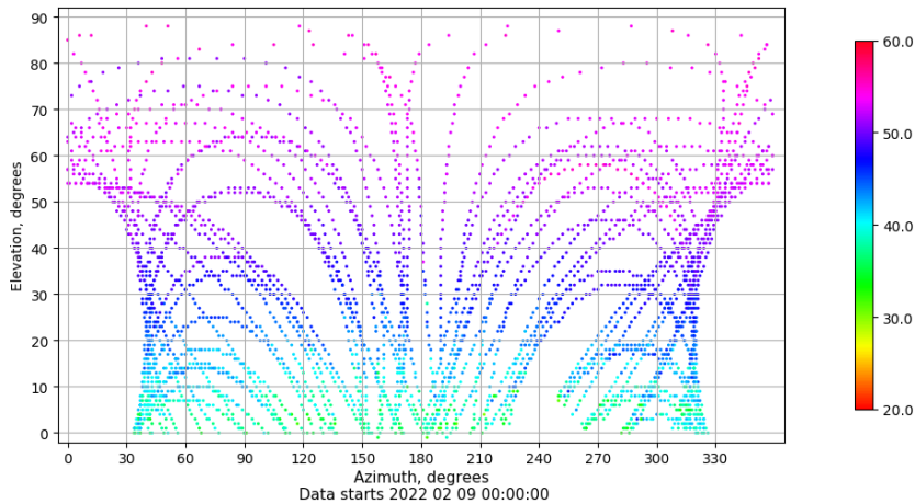
Azimuth-elevation plot for station IZAN. Signal to Noise S1C Data file IZAN00ESP_R_2022040.xtr
