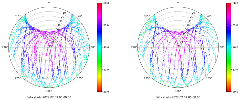
Skyplot for station IZAN. Signal to Noise S1C Data file IZAN00ESP_R_2022040.xtr Skyplot for station IZAN. Signal to Noise S2S Data file IZAN00ESP_R_2022040.xtr
