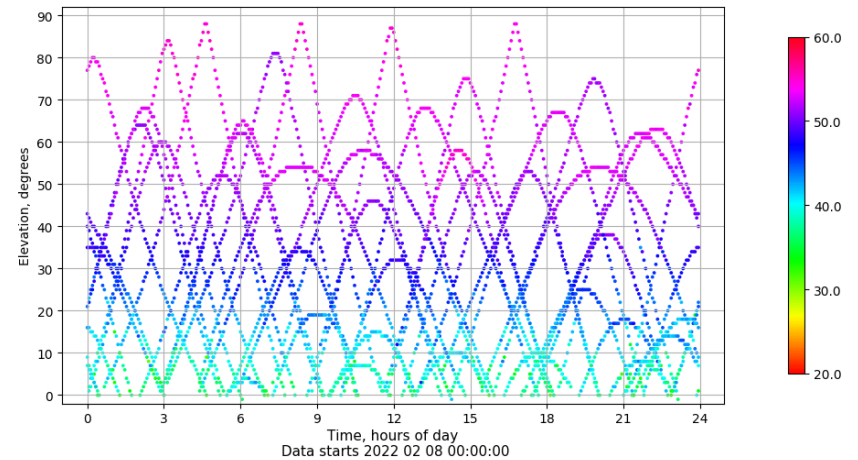
Time-elevation plot for station IZAN. Signal to Noise S1C Data file IZAN00ESP_R_2022039.xtr
