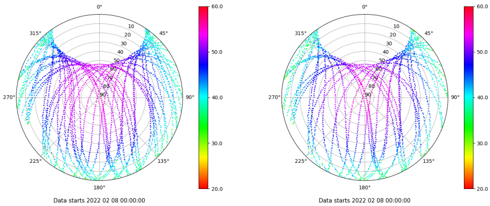
Skyplot for station IZAN. Signal to Noise S1C Data file IZAN00ESP_R_2022039.xtr Skyplot for station IZAN. Signal to Noise S2S Data file IZAN00ESP_R_2022039.xtr
