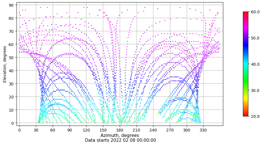
Azimuth-elevation plot for station IZAN. Signal to Noise S1C Data file IZAN00ESP_R_2022039.xtr
