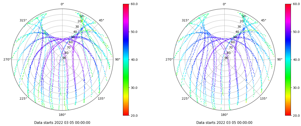
Skyplot for station HUE1. Signal to Noise S1C Data file HUE100ESP_R_2022064.xtr Skyplot for station HUE1. Signal to Noise S2P Data file HUE100ESP_R_2022064.xtr
