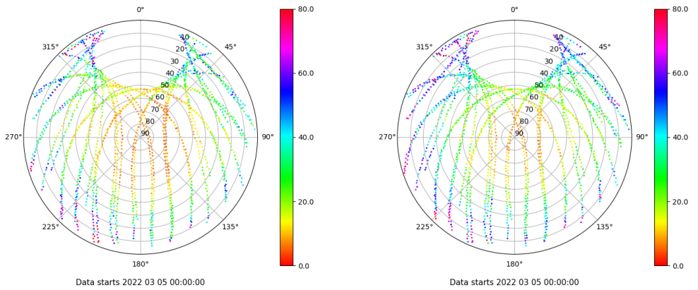
Skyplot for station HUE1. Parameter M1C Data file HUE100ESP_R_2022064.xtr Skyplot for station HUE1. Parameter M2P Data file HUE100ESP_R_2022064.xtr
