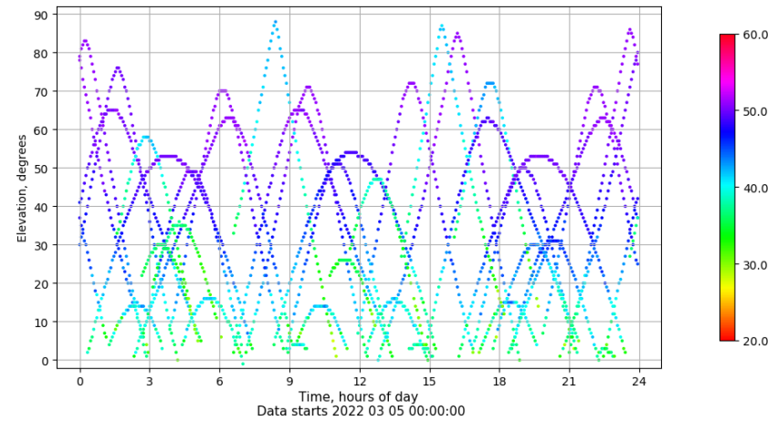
Time-elevation plot for station HUE1. Signal to Noise S1C Data file HUE100ESP_R_2022064.xtr
