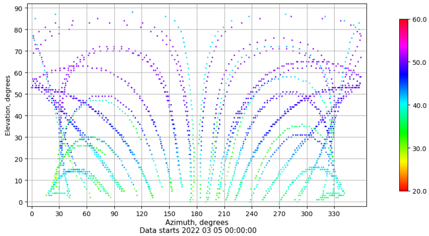
Azimuth-elevation plot for station HUE1. Signal to Noise S1C Data file HUE100ESP_R_2022064.xtr
