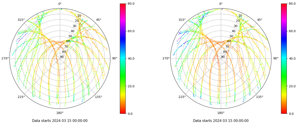
Skyplot for station GIRO. Parameter M1C Data file GIRO00ESP_R_2024075.xtr Skyplot for station GIRO. Parameter M2P Data file GIRO00ESP_R_2024075.xtr
