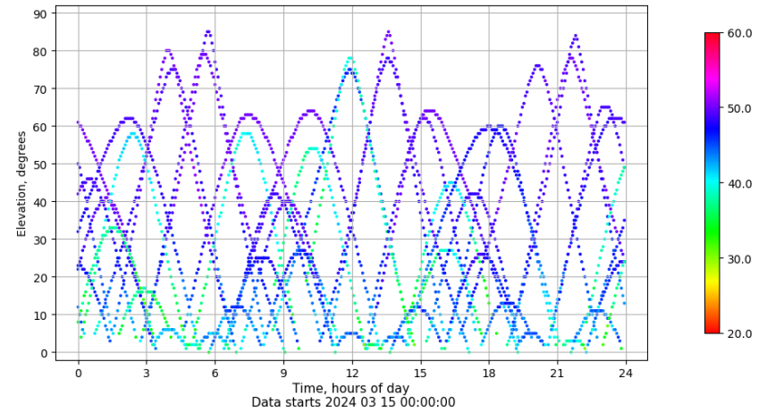
Time-elevation plot for station GIRO. Signal to Noise S1C Data file GIRO00ESP_R_2024075.xtr
