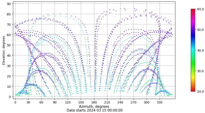
Azimuth-elevation plot for station GIRO. Signal to Noise S1C Data file GIRO00ESP_R_2024075.xtr
