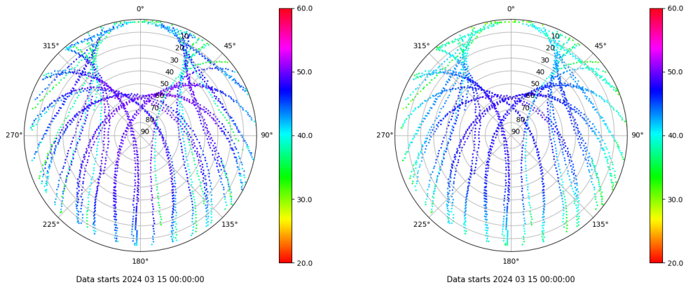
Skyplot for station GIRO. Signal to Noise S1C Data file GIRO00ESP_R_2024075.xtr Skyplot for station GIRO. Signal to Noise S2P Data file GIRO00ESP_R_2024075.xtr
