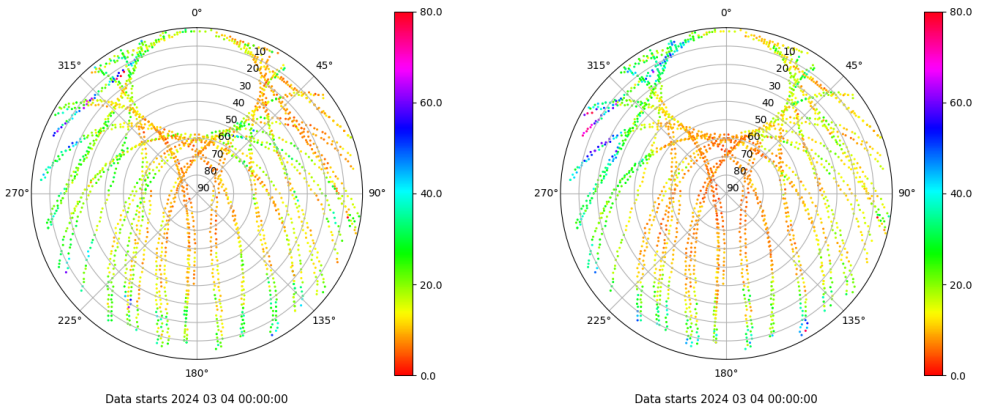
Skyplot for station GIRO. Parameter M1C Data file GIRO00ESP_R_2024064.xtr Skyplot for station GIRO. Parameter M2P Data file GIRO00ESP_R_2024064.xtr
