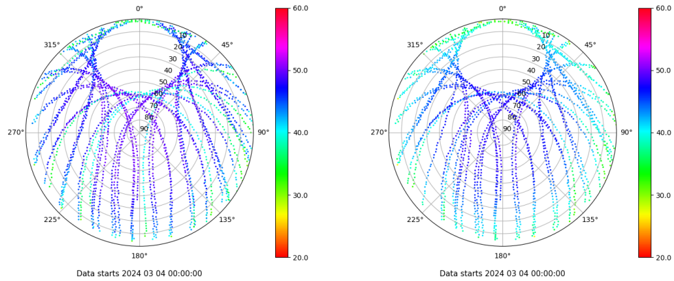
Skyplot for station GIRO. Signal to Noise S1C Data file GIRO00ESP_R_2024064.xtr Skyplot for station GIRO. Signal to Noise S2P Data file GIRO00ESP_R_2024064.xtr
