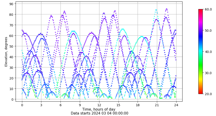
Time-elevation plot for station GIRO. Signal to Noise S1C Data file GIRO00ESP_R_2024064.xtr
