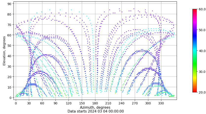
Azimuth-elevation plot for station GIRO. Signal to Noise S1C Data file GIRO00ESP_R_2024064.xtr
