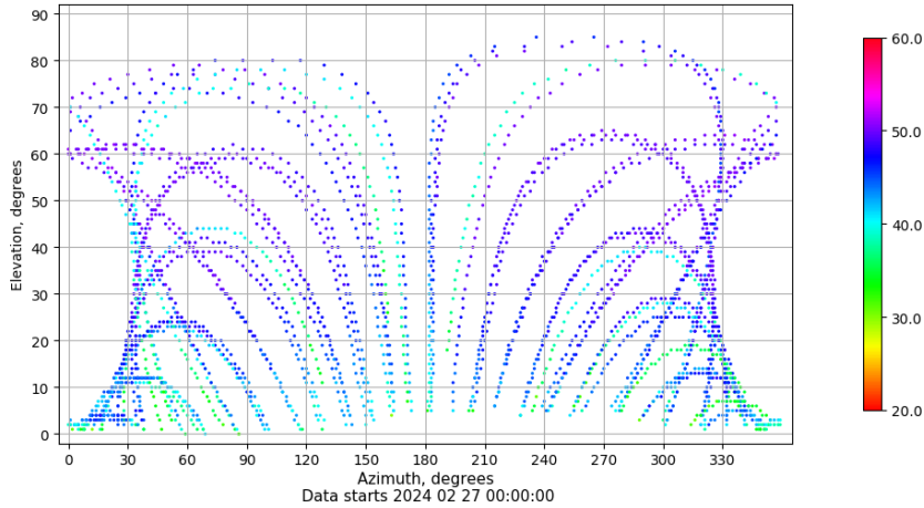
Azimuth-elevation plot for station GIRO. Signal to Noise S1C Data file GIRO00ESP_R_2024058.xtr
