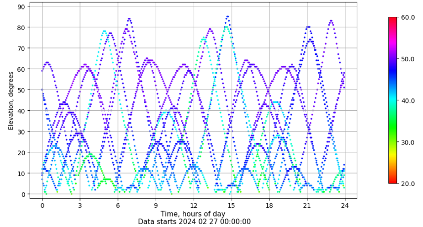
Time-elevation plot for station GIRO. Signal to Noise S1C Data file GIRO00ESP_R_2024058.xtr
